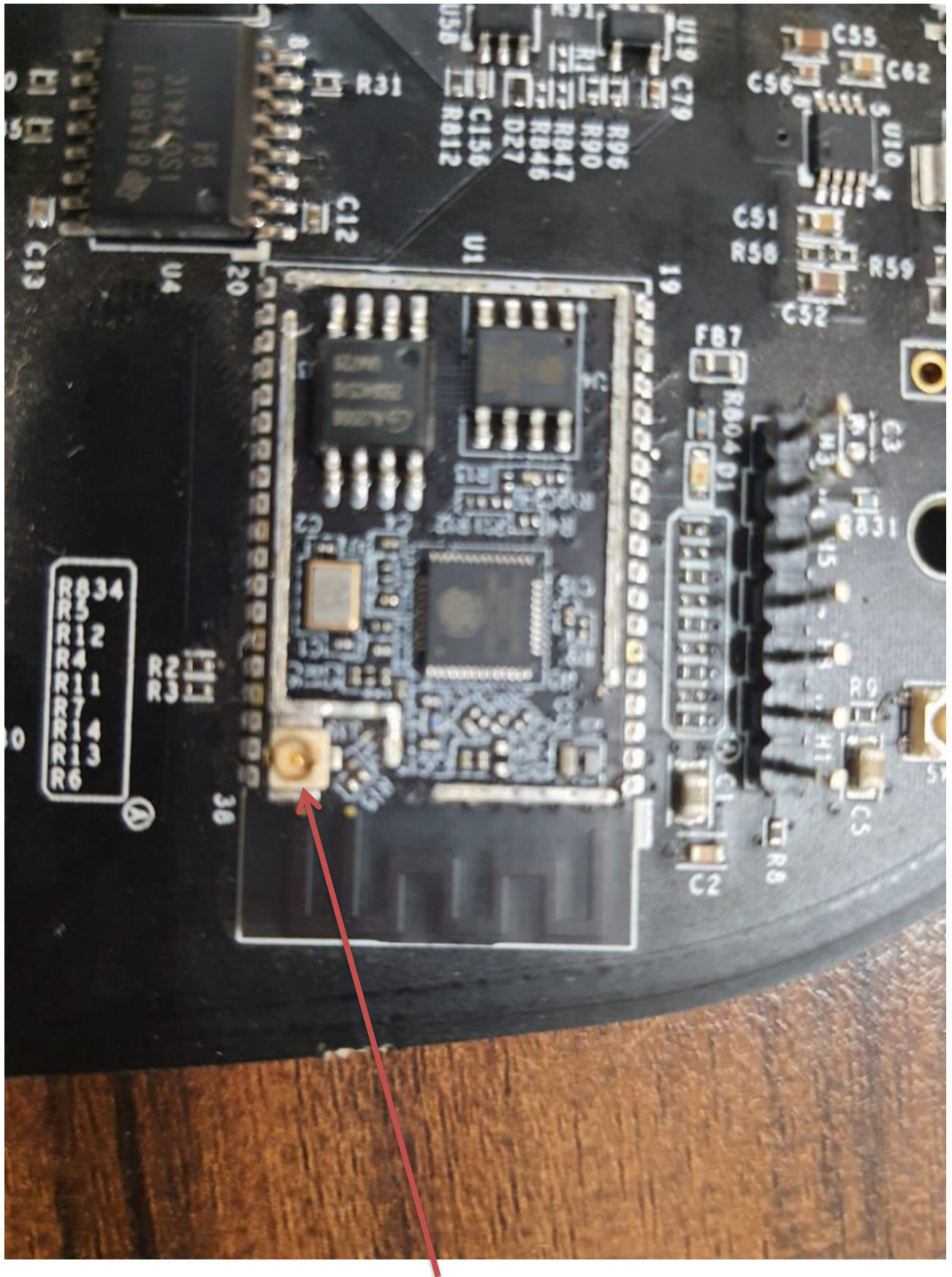
Antenna Port 2.4g Wifi
