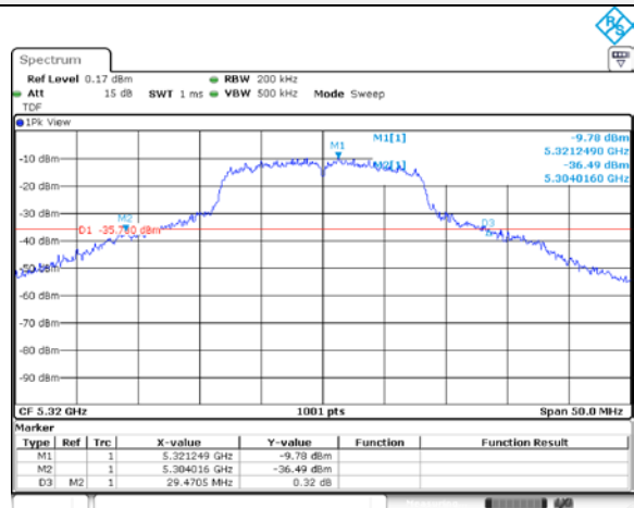
UNII-2A / 802.11a / High ch.
