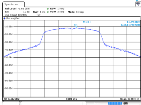
UNII-2A / 802.11a / Mid ch.
