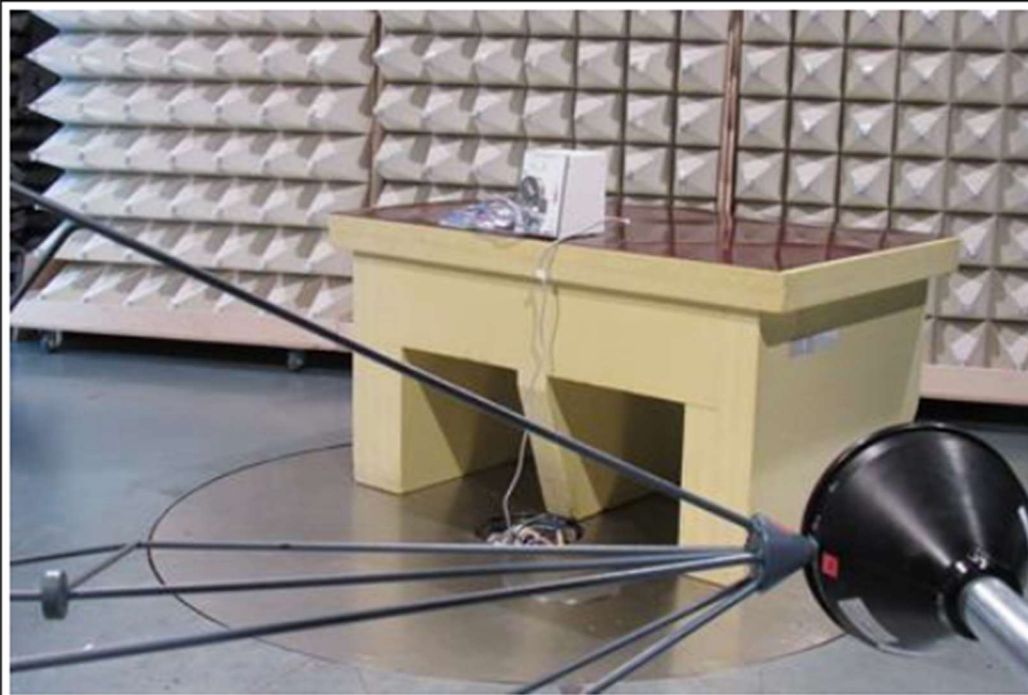
Setup Radiated Emission 1
