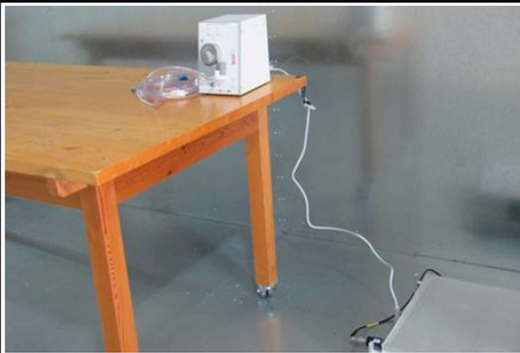
Setup Conducted Emission
