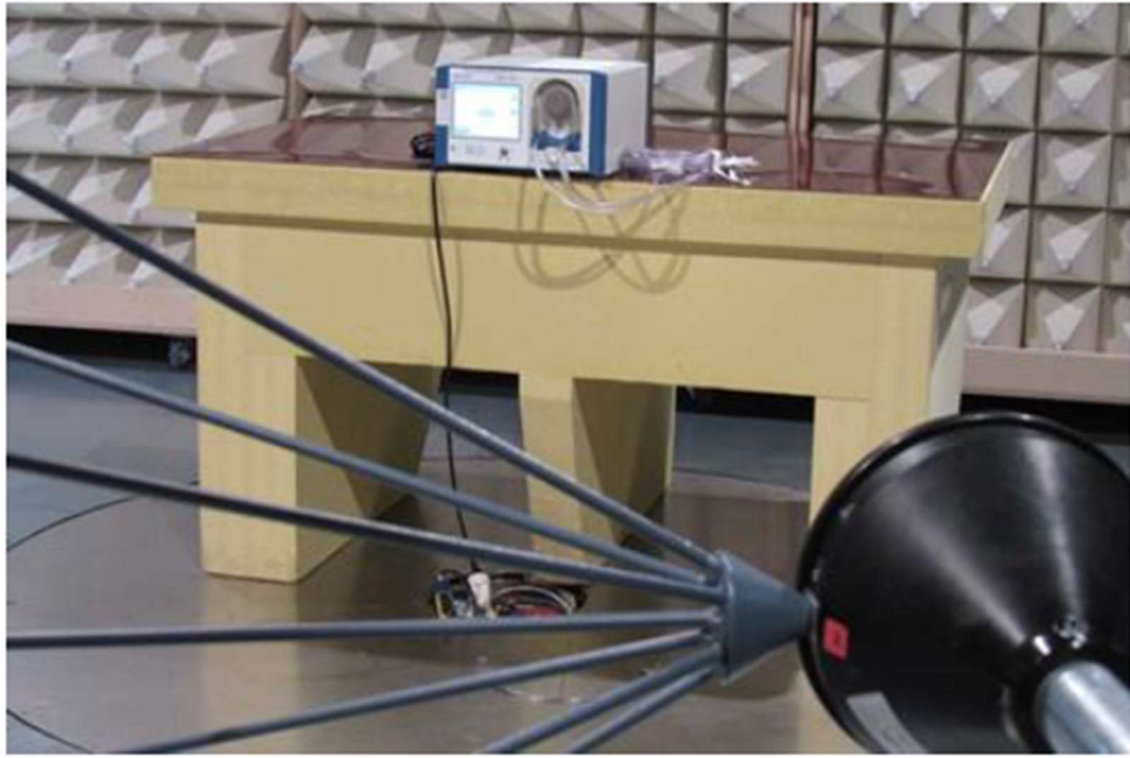
Radiated Setup 1
