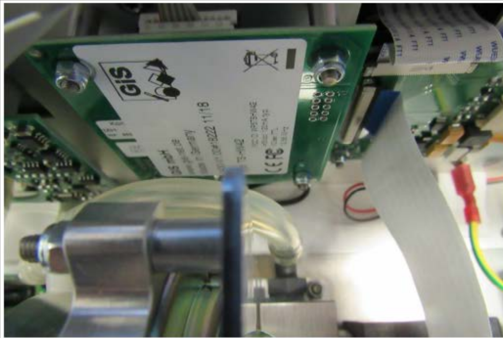
EUT Internal Architecture View 3
