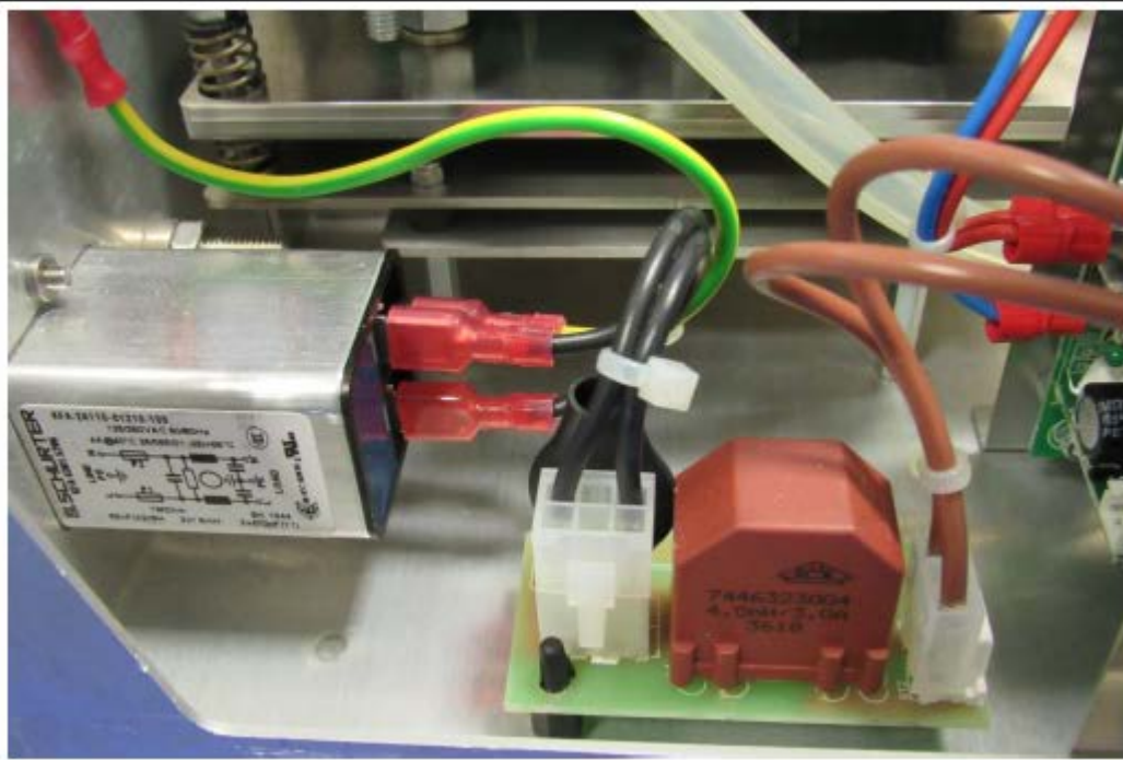
EUT Internal Architecture View 14
