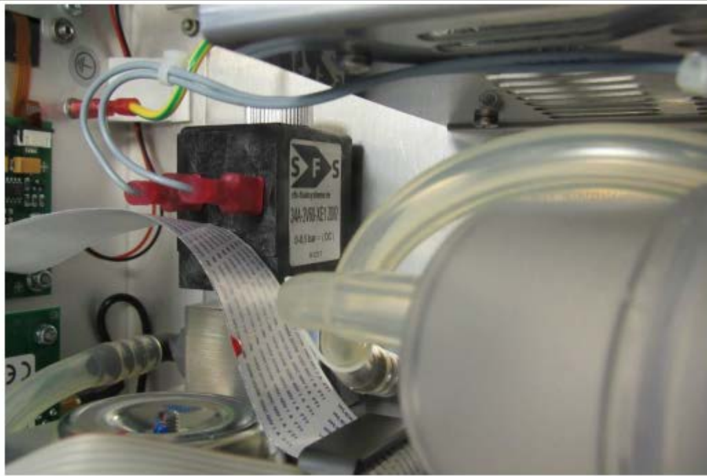
EUT Internal Architecture View 13
