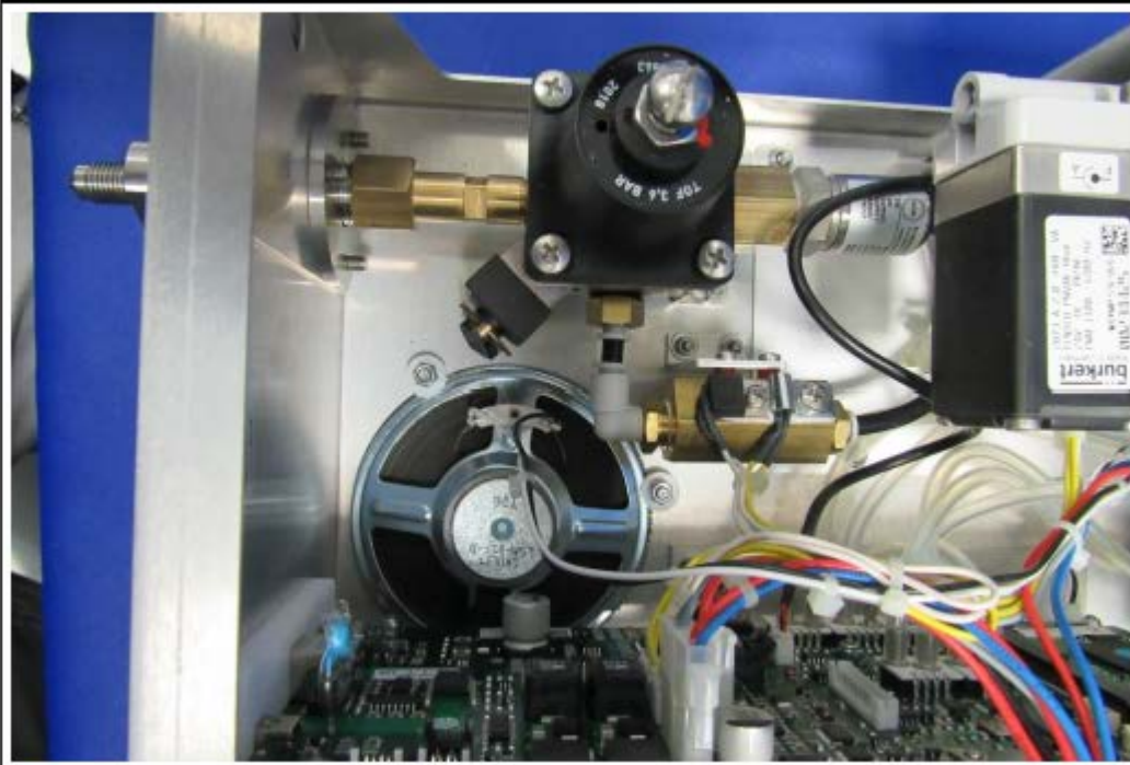
EUT Internal Architecture View 8
