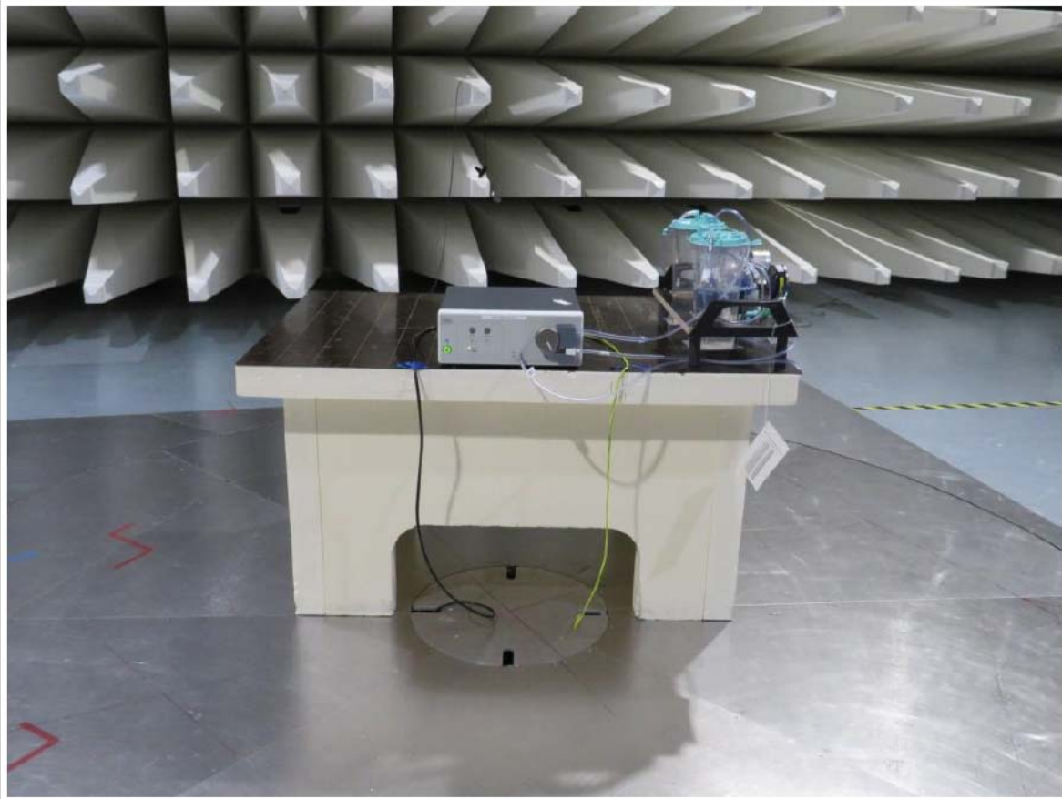
Test Setup Picture 2
