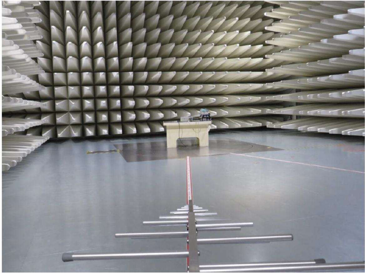
Test Setup Picture 1
