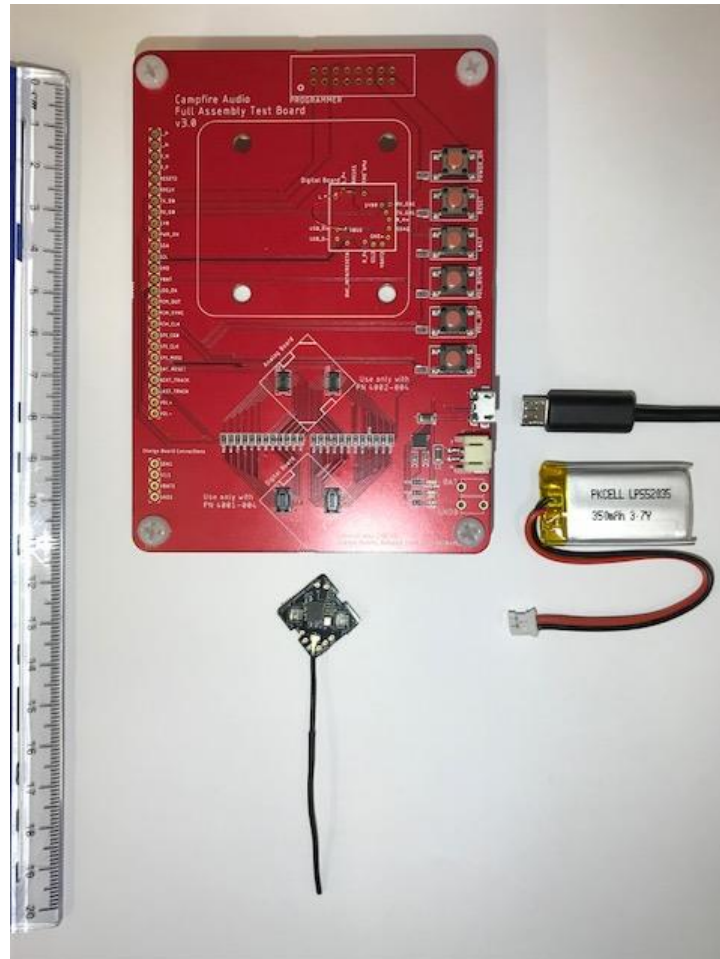
Figure 4: External Photo Campfire BT Yoke 4000 – Auxiliary board for radio configuration – Top
