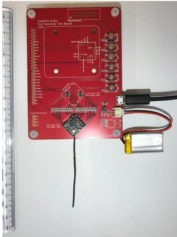
Figure 5: External Photo Campfire BT Yoke 4000 – Auxiliary board for radio configuration mounted – top
