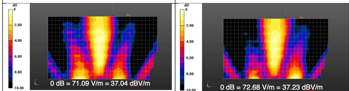
Figure 11: Unobstructed E-field scan at 1 m behind Client – Horiz. Plane (Normalized to peak field strength behind client of 71.09 V/m)
