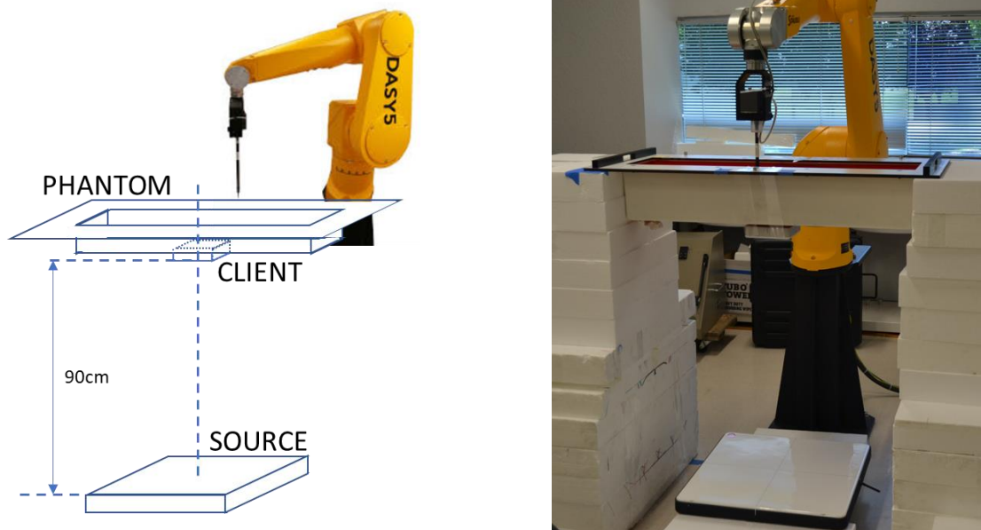
Figure 16 - SAR measurement test setup
