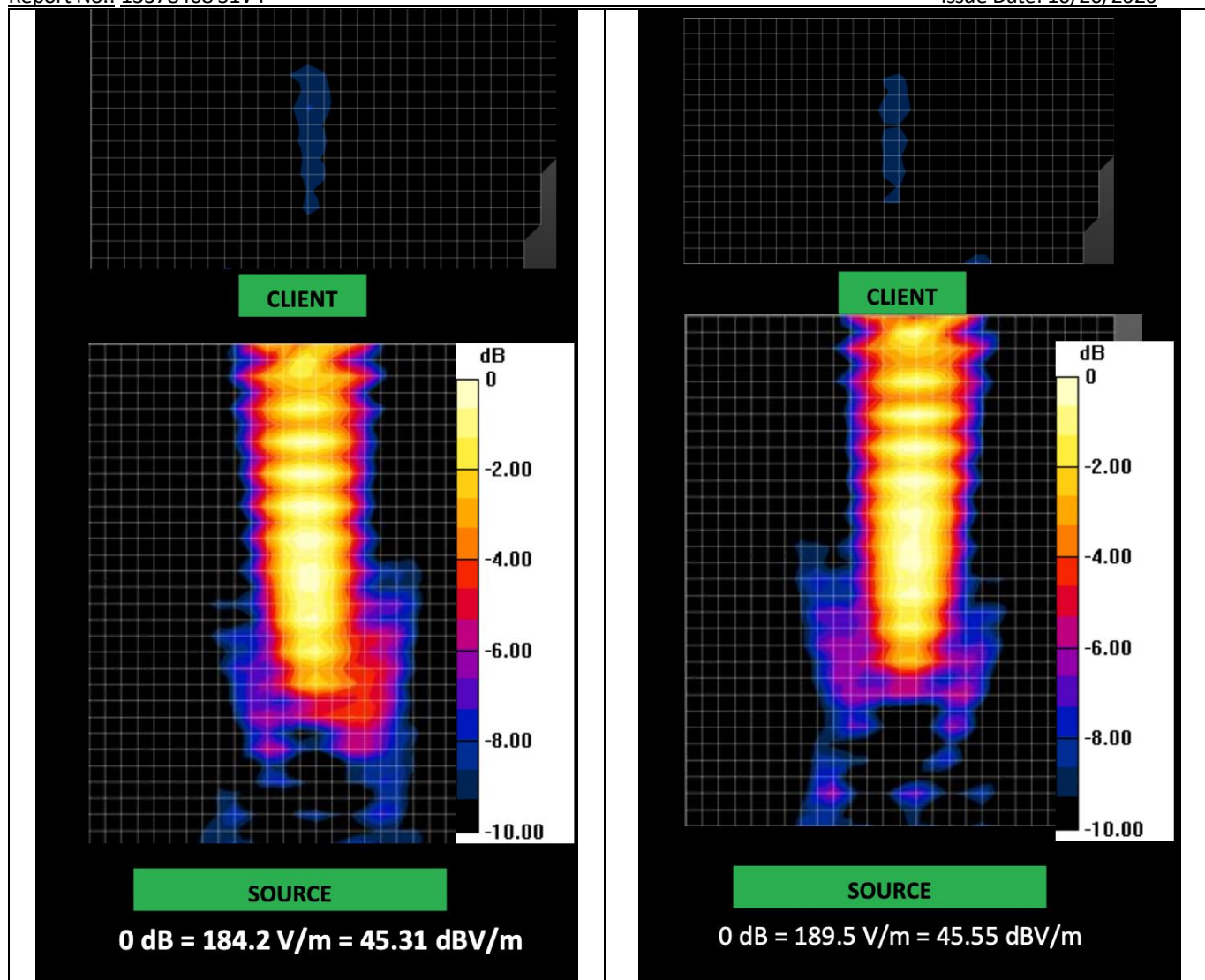
Figure 9 Unobstructed E-field scan at 1 m between Source and Client - Horizontal Plane
