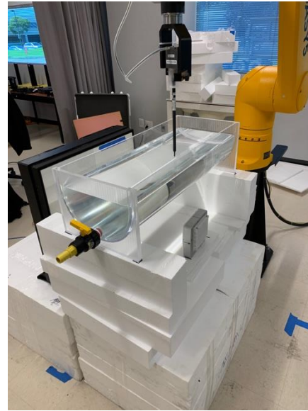
Figure 87: Half-cylinder phantom - partial obstruction
