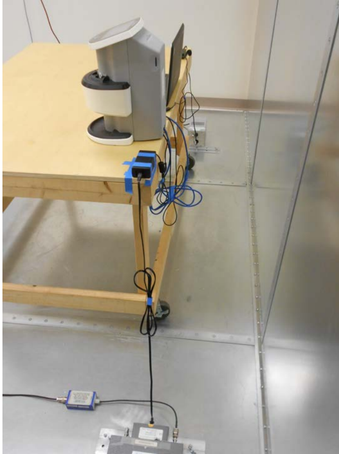
LINE CONDUCTED EMISSION (BACK)
