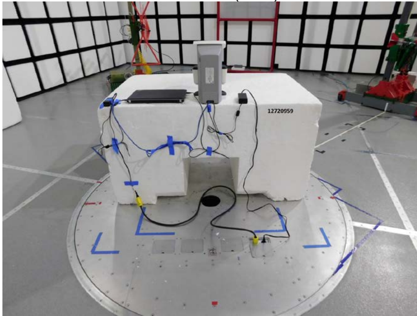
RADIATED EMISSIONS BELOW 1GHz (BACK)
