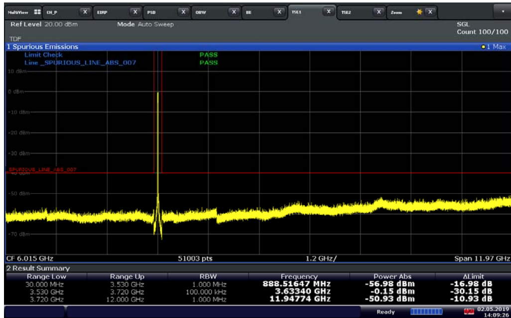
LTE Band 48 / 20 MHz / QPSK – Mid Channel_1
