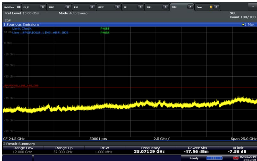
LTE Band 48 / 20 MHz / QPSK – Mid Channel_2
