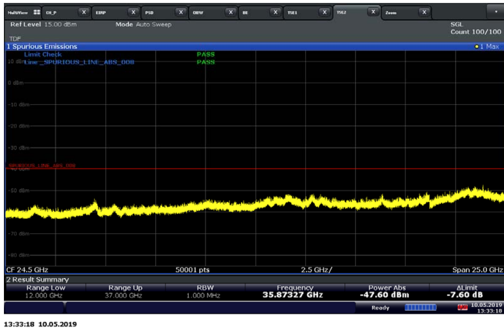
LTE Band 48 / 10 MHz / 64QAM – Mid Channel_2
