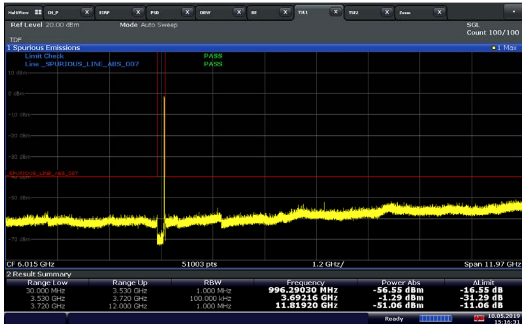
LTE Band 48 / 10 MHz / QPSK – High Channel_1
