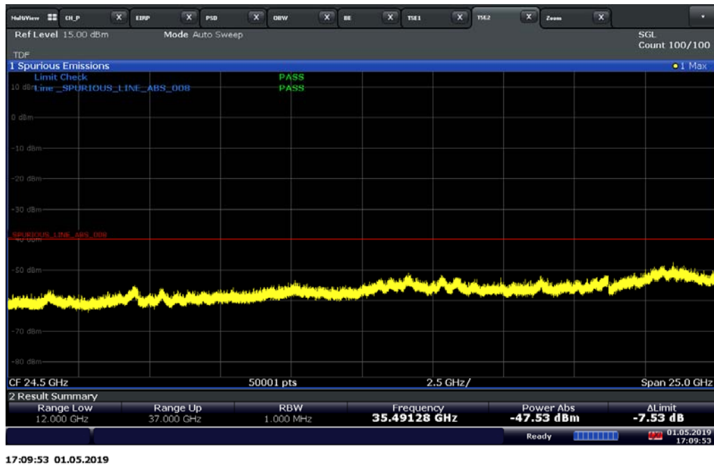
LTE Band 48 / 20 MHz / 16QAM – Mid Channel_2
