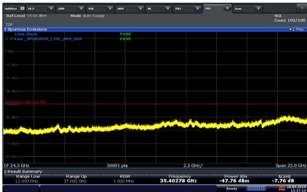
LTE Band 48 / 10 MHz / QPSK – High Channel_2
