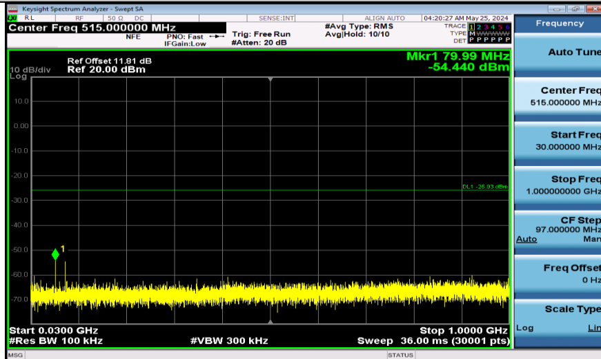
11B-Ant1-2462-30~1000-PASS
