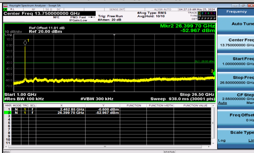
11G-Ant1-2462-1000~26500-PASS
