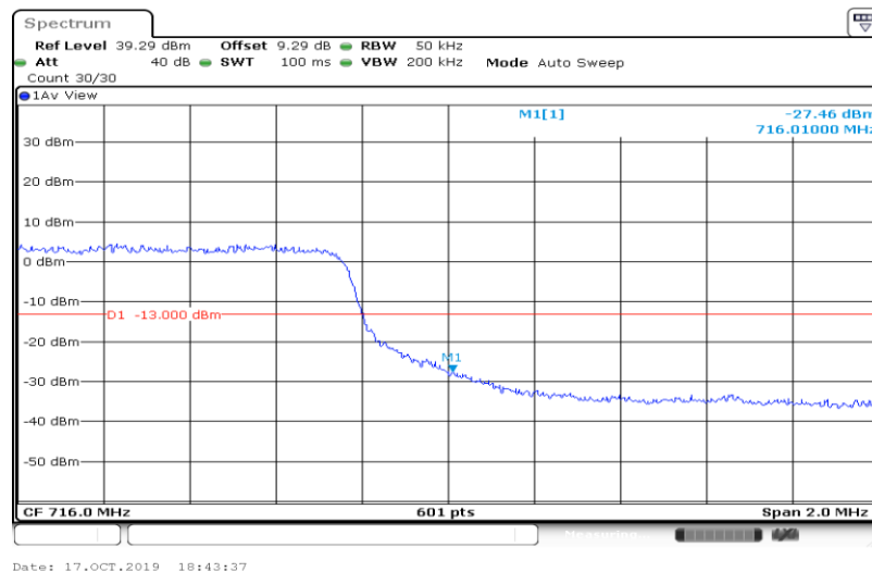
Band17-10MHz-QPSK-23780-1RB#49
