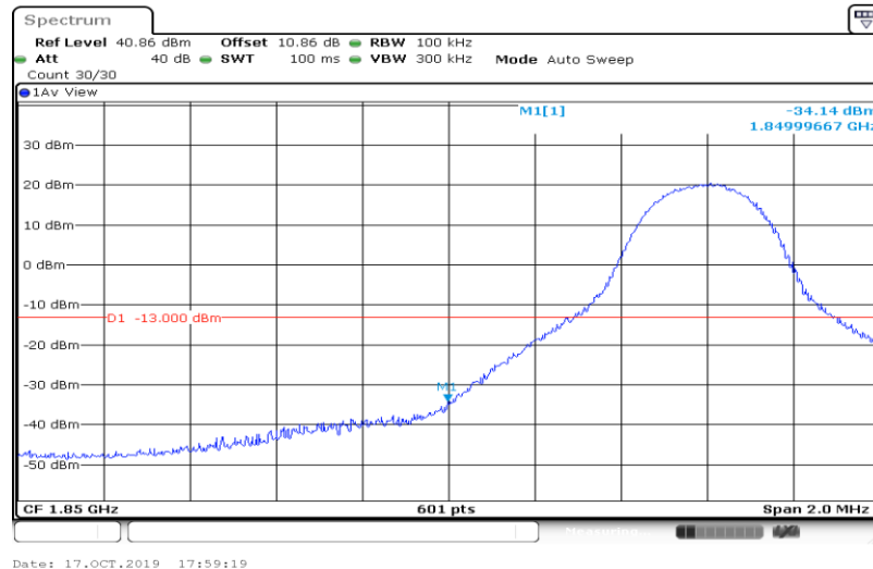
Band2-10MHz-16QAM-18650-1RB#49
