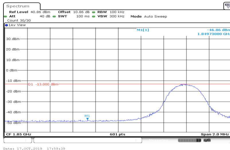
Band2-10MHz-16QAM-18650-50RB#0
