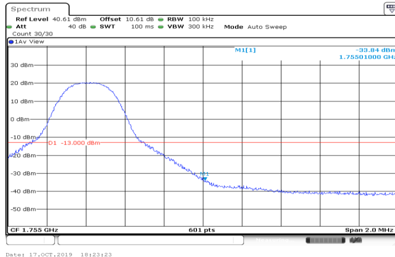
Band4-10MHz-16QAM-20350-1RB#0
