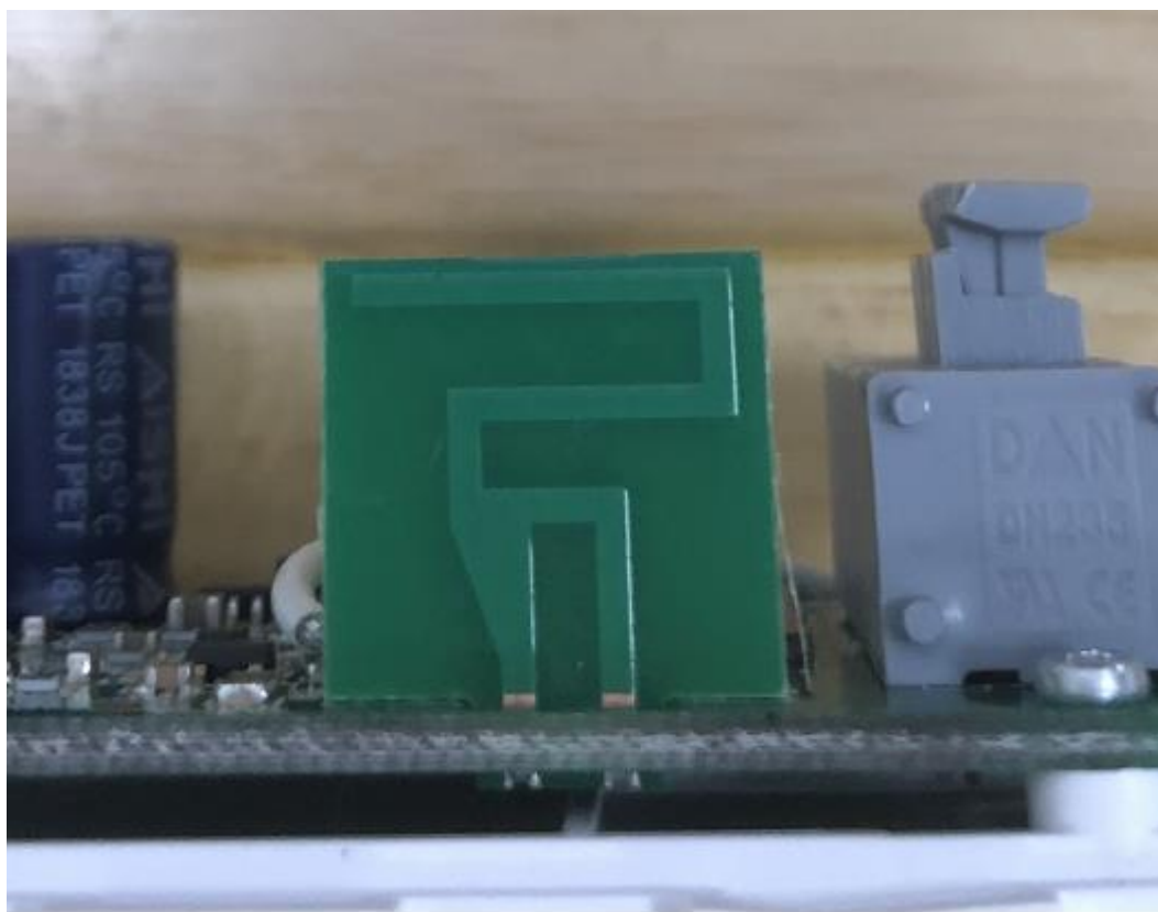
Detail View of Antenna
