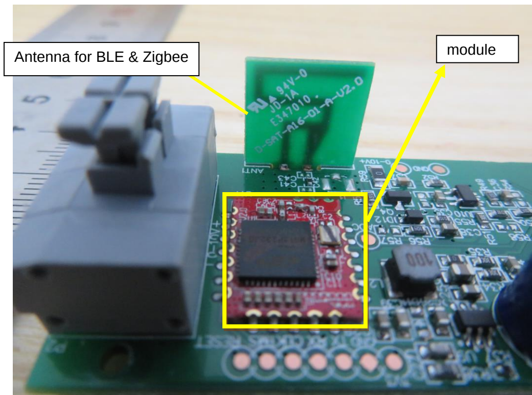
Detail View of Antenna
