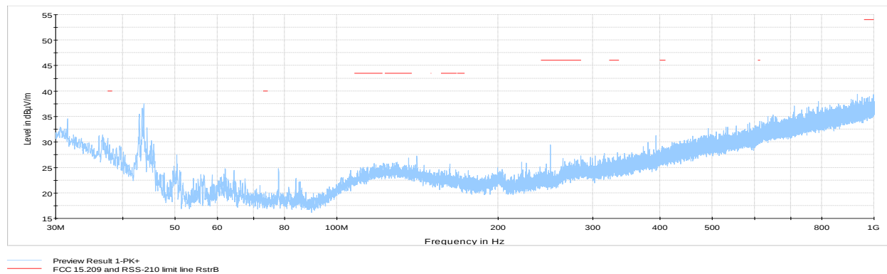
Figure 8.7-48: Cabinet radiated Spurious emissions within 30 to 1000 MHz, Tx @ high channel
