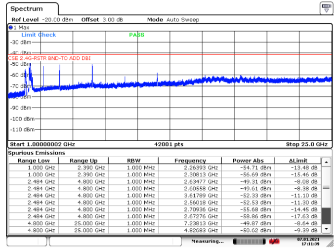
Figure 8.7-41: Conducted spurious emissions above 1 GHz within restricted bands, Tx on low channel of 802.11n
