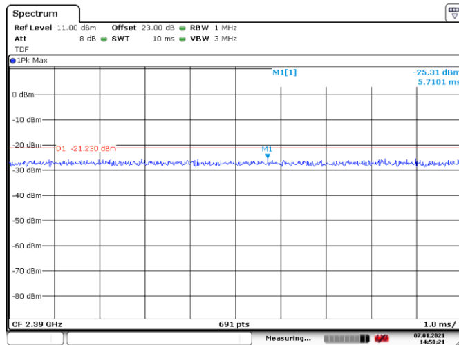
Figure 8.7-20: Conducted spurious emissions on 2390 MHz, peak, Tx on 802.11g
