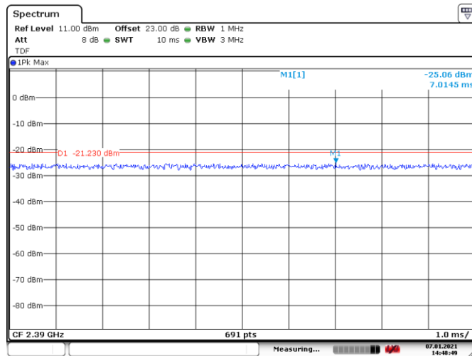
Figure 8.7-24: Conducted spurious emissions on 2390 MHz, peak, Tx on 802.11n
