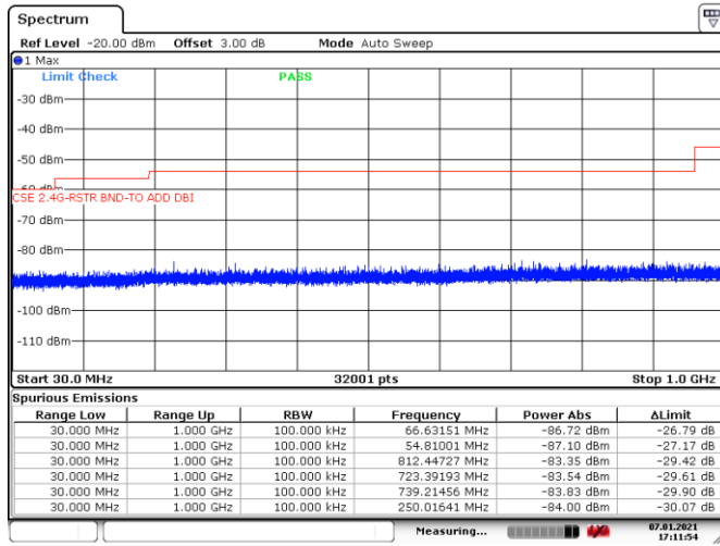
Figure 8.7-40: Conducted spurious emissions 30 MHz to 1 GHz within restricted bands, Tx on low channel of 802.11n
