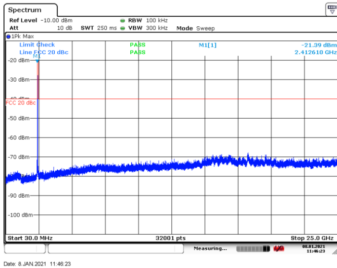
Figure 8.7-7: Conducted spurious emissions, tx on low channel, Tx on 802.11b
