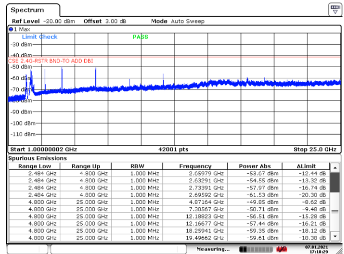
Figure 8.7-37: Conducted spurious emissions above 1 GHz within restricted bands, Tx on mid channel of 802.11g
