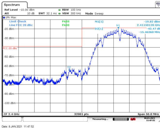
Figure 8.7-1: Conducted Band edge spurious emissions at 2400 MHz, Tx on 802.11b
