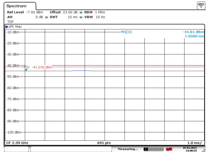
Figure 8.7-21: Conducted spurious emissions on 2390 MHz, average, Tx on 802.11g
