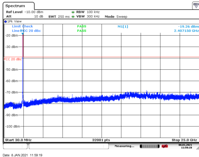
Figure 8.7-13: Conducted spurious emissions, tx on low channel, Tx on 802.11n
