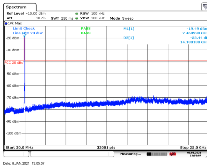
Figure 8.7-15: Conducted spurious emissions, tx on high channel, Tx on 802.11n
