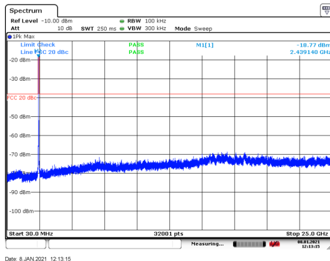
Figure 8.7-11: Conducted spurious emissions, tx on mid channel, Tx on 802.11g
