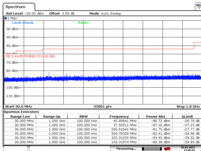
Figure 8.7-30: Conducted spurious emissions 30 MHz to 1 GHz within restricted bands, Tx on mid channel of 802.11b
