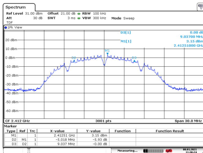
Figure 8.8-1: PSD on 802.11b, sample plot
