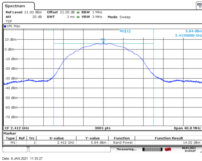
Figure 8.6-1: Output power on 802.11b, sample plot
