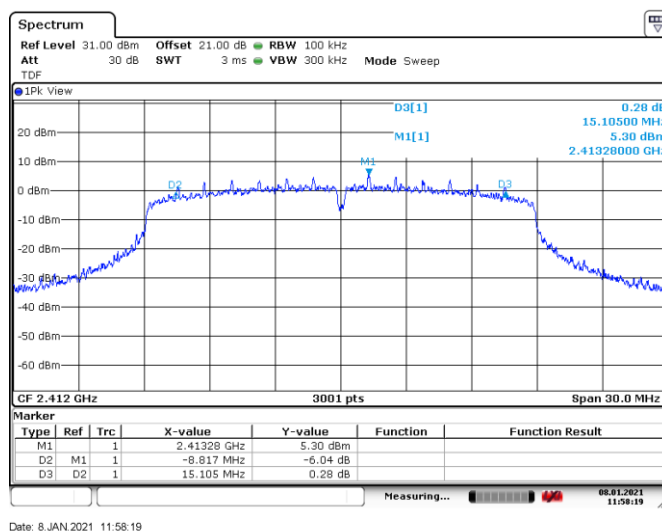
Figure 8.5-3: 6 dB bandwidth on 802.11n, sample plot
