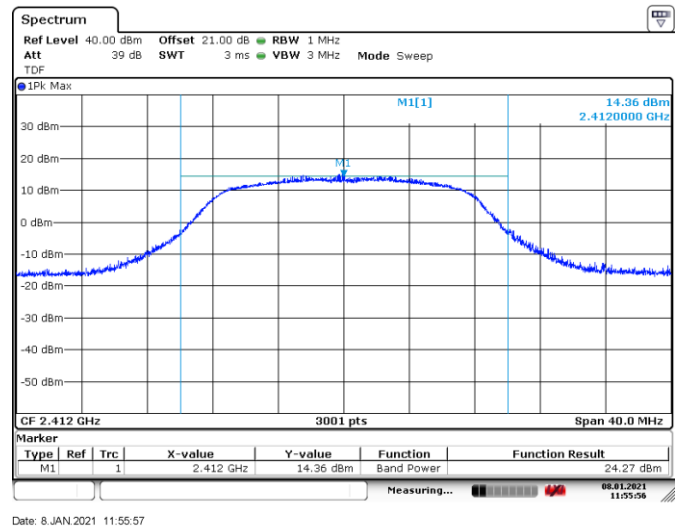
Figure 8.6-2: Output power on 802.11g, sample plot
