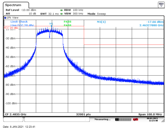
Figure 8.7-4: Conducted Band edge spurious emissions at 2483.5 MHz, Tx on 802.11b
