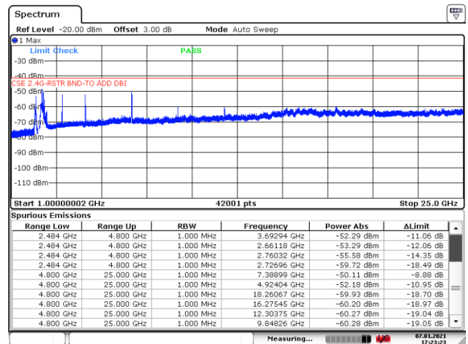
Figure 8.7-39: Conducted spurious emissions above 1 GHz within restricted bands, Tx on high channel of 802.11g
