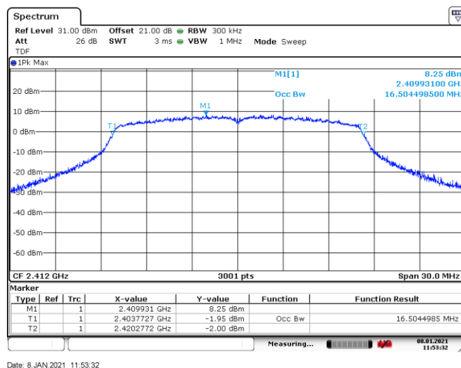
Figure 8.5-5: 99% occupied bandwidth on 802.11g, sample plot
