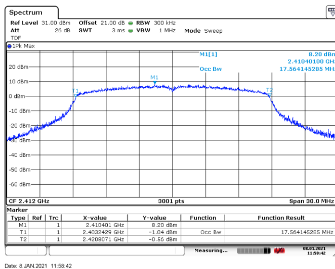
Figure 8.5-6: 99% occupied bandwidth on 802.11n, sample plot
