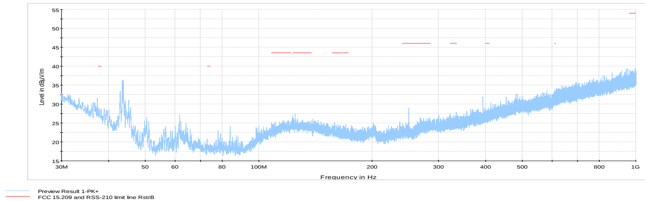
Figure 8.7-46: Cabinet radiated Spurious emissions within 30 to 1000 MHz, Tx @ low channel
