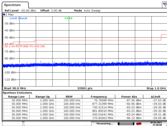
Figure 8.7-36: Conducted spurious emissions 30 MHz to 1 GHz within restricted bands, Tx on mid channel of 802.11g
