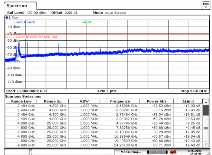
Figure 8.7-43: Conducted spurious emissions above 1 GHz within restricted bands, Tx on mid channel of 802.11n
