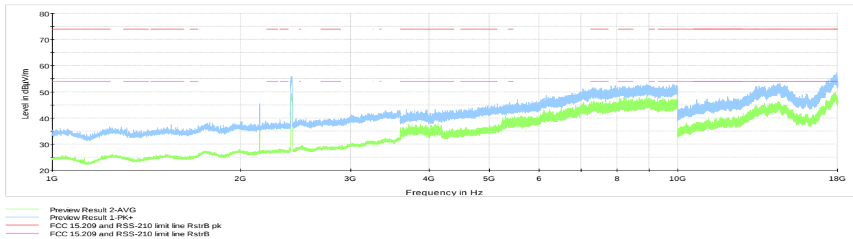
Figure 8.7-49: Cabinet radiated Spurious emissions 1to18 GHz, Tx @ low channel
