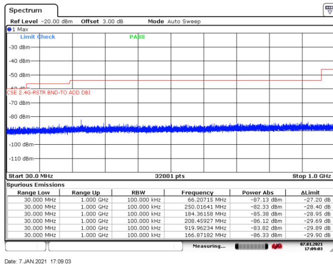
Figure 8.7-34: Conducted spurious emissions 30 MHz to 1 GHz within restricted bands, Tx on low channel of 802.11g
