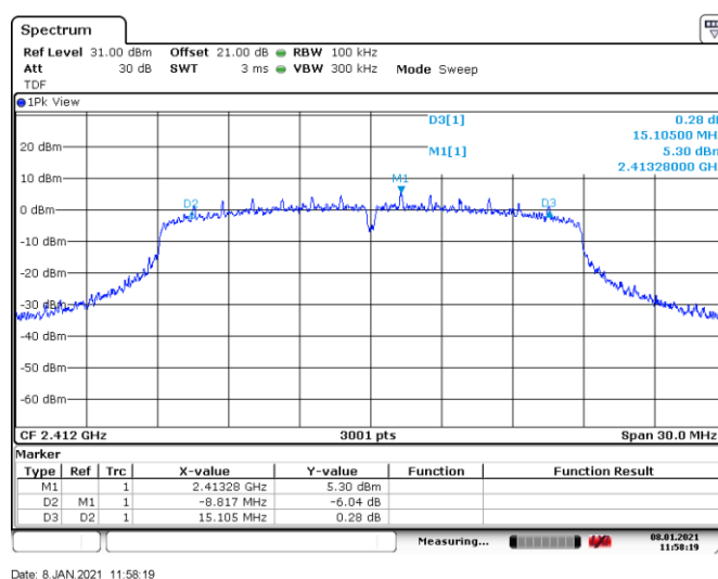
Figure 8.8-3: PSD on 802.11n, sample plot
