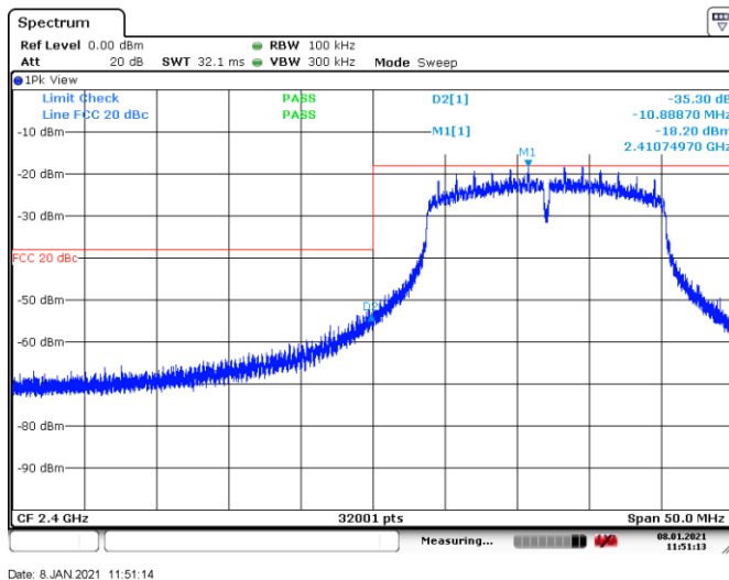
Figure 8.7-3: Conducted Band edge spurious emissions at 2400 MHz, Tx on 802.11b
