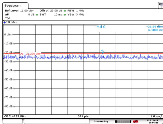
Figure 8.7-22: Conducted spurious emissions on 2483.5MHz, peak, Tx on 802.11g
