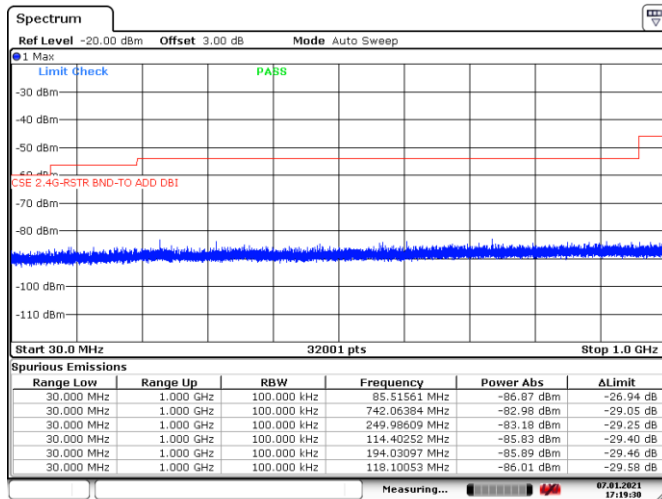
Figure 8.7-42: Conducted spurious emissions 30 MHz to 1 GHz within restricted bands, Tx on mid channel of 802.11n
