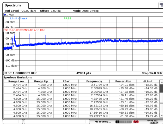
Figure 8.7-29: Conducted spurious emissions above 1 GHz within restricted bands, Tx on low channel of 802.11b
