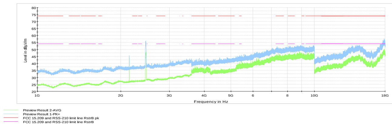
Figure 8.7-51: Cabinet radiated Spurious emissions 1to18 GHz, Tx @ high channel
