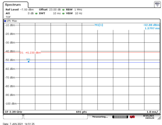
Figure 8.7-17: Conducted spurious emissions on 2390 MHz, average, Tx on 802.11b
