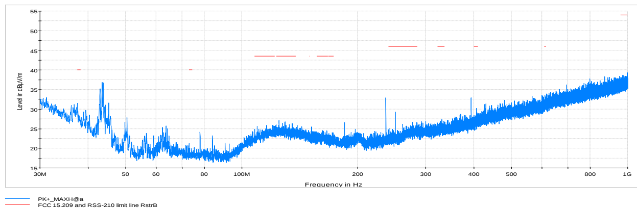
Figure 8.7-47: Cabinet radiated Spurious emissions within 30 to 1000 MHz, Tx @ mid channel
