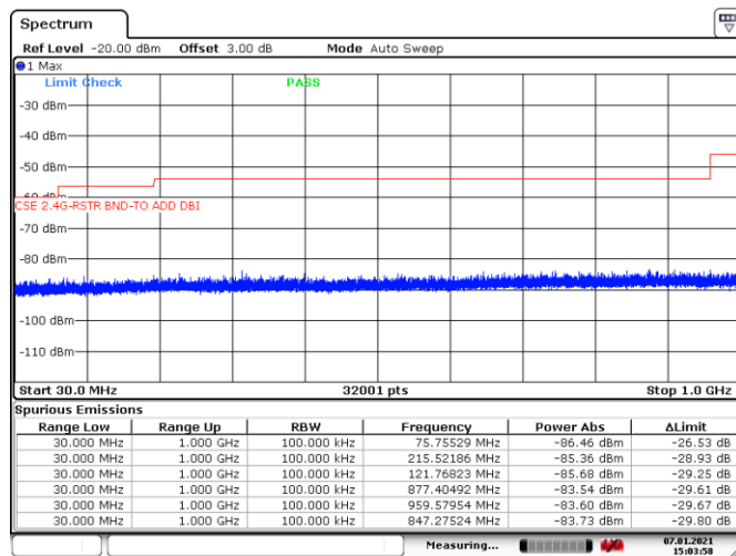
Figure 8.7-28: Conducted spurious emissions 30 MHz to 1 GHz within restricted bands, Tx on low channel of 802.11b
