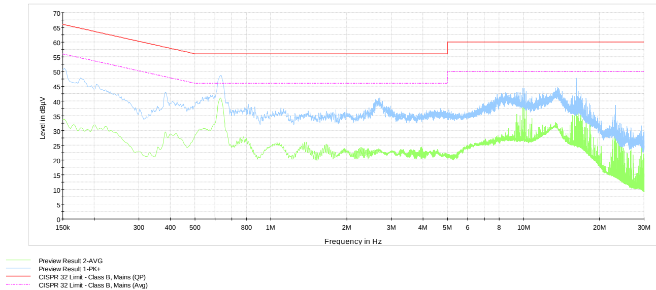
Plot 8.4-1: Conducted emissions on phase line
