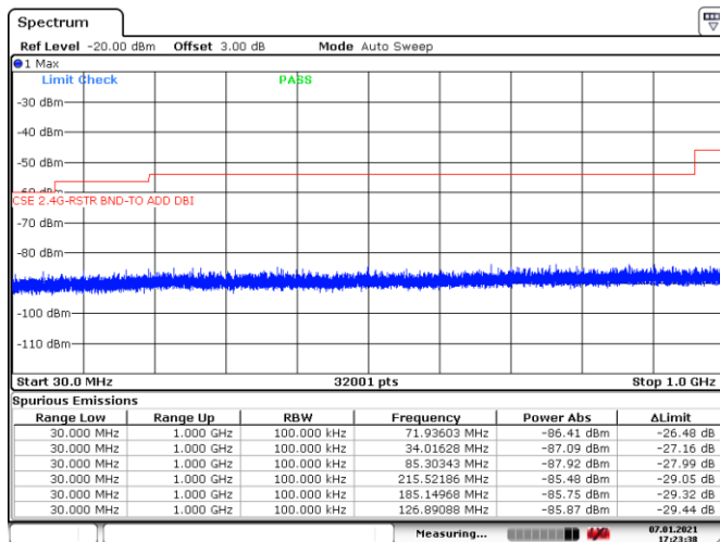
Figure 8.7-38: Conducted spurious emissions 30 MHz to 1 GHz within restricted bands, Tx on high channel of 802.11g
