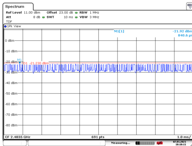
Figure 8.7-26: Conducted spurious emissions on 2483.5 MHz, peak, Tx on 802.11n
