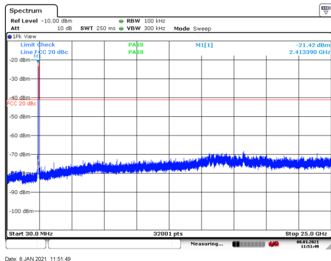
Figure 8.7-10: Conducted spurious emissions, tx on low channel, Tx on 802.11g
