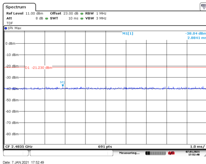
Figure 8.7-18: Conducted spurious emissions on 2483.5MHz, peak, Tx on 802.11b
