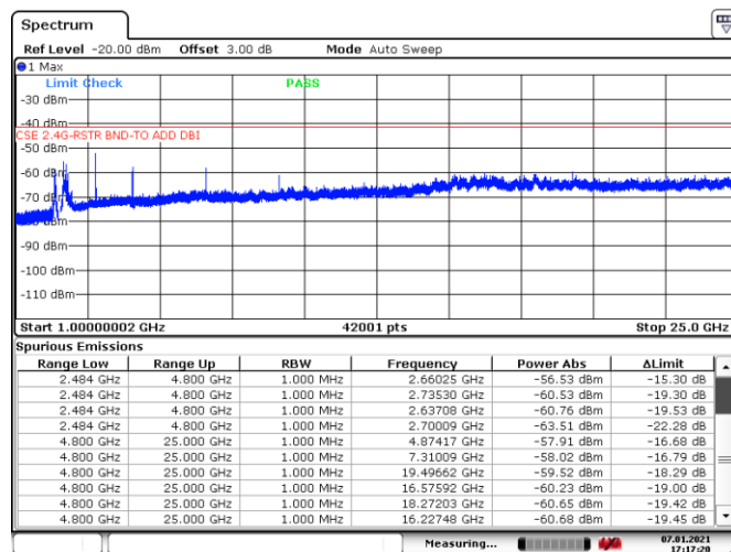
Figure 8.7-31: Conducted spurious emissions above 1 GHz within restricted bands, Tx on mid channel of 802.11b
