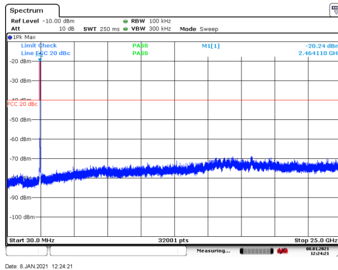
Figure 8.7-9: Conducted spurious emissions, tx on high channel, Tx on 802.11b
