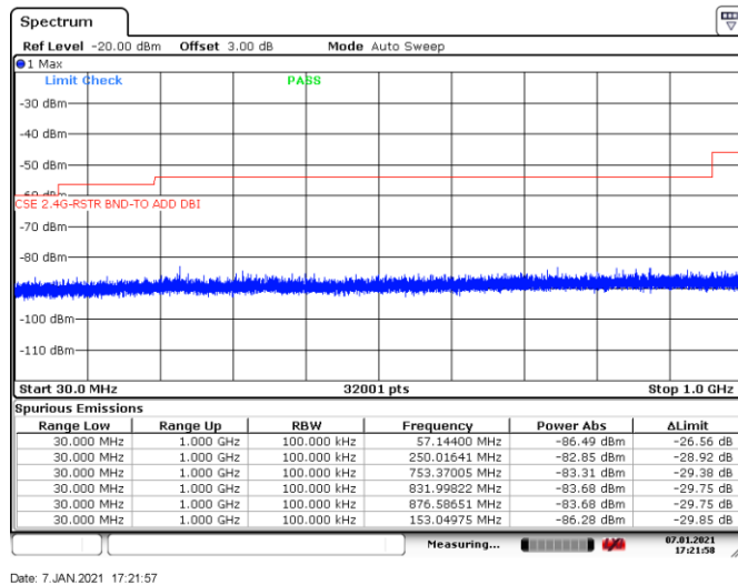
Figure 8.7-32: Conducted spurious emissions 30 MHz to 1 GHz within restricted bands, Tx on high channel of 802.11b
