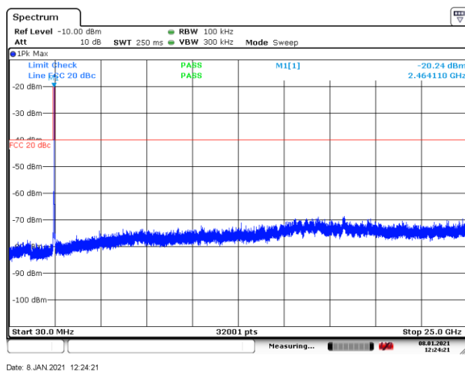
Figure 8.7-12: Conducted spurious emissions, tx on high channel, Tx on 802.11g
