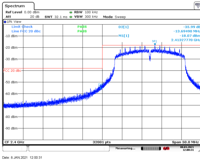
Figure 8.7-5: Conducted Band edge spurious emissions at 2400 MHz, Tx on 802.11n
