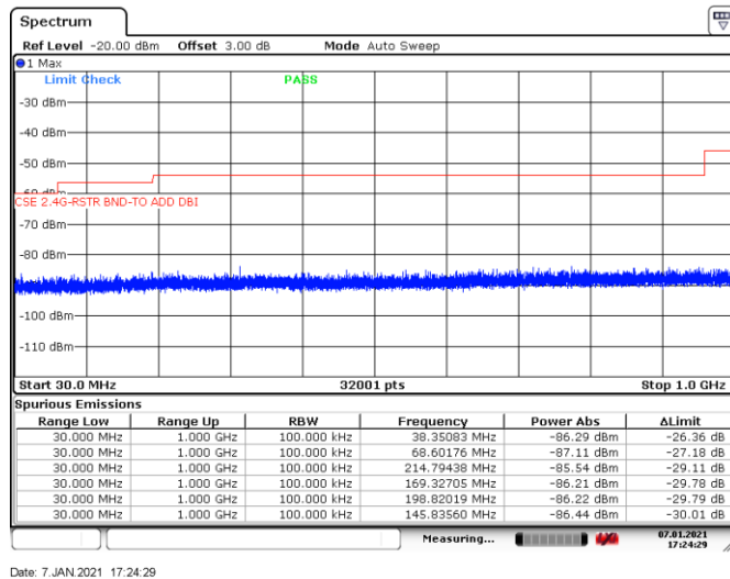
Figure 8.7-44: Conducted spurious emissions 30 MHz to 1 GHz within restricted bands, Tx on high channel of 802.11n
