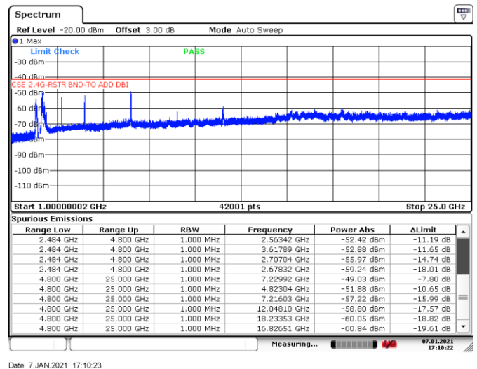
Figure 8.7-35: Conducted spurious emissions above 1 GHz within restricted bands, Tx on low channel of 802.11g
