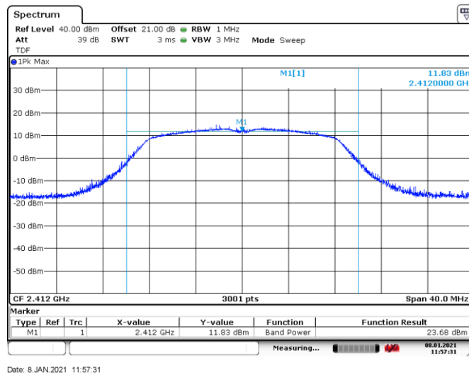
Figure 8.6-3: Output power on 802.11n, sample plot
