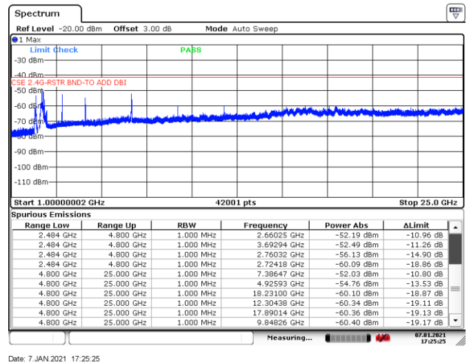
Figure 8.7-45: Conducted spurious emissions above 1 GHz within restricted bands, Tx on high channel of 802.11n
