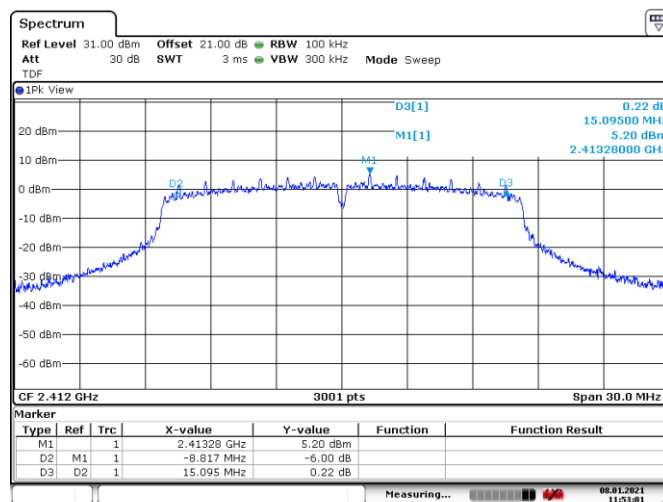
Figure 8.8-2: PSD on 802.11g, sample plot
