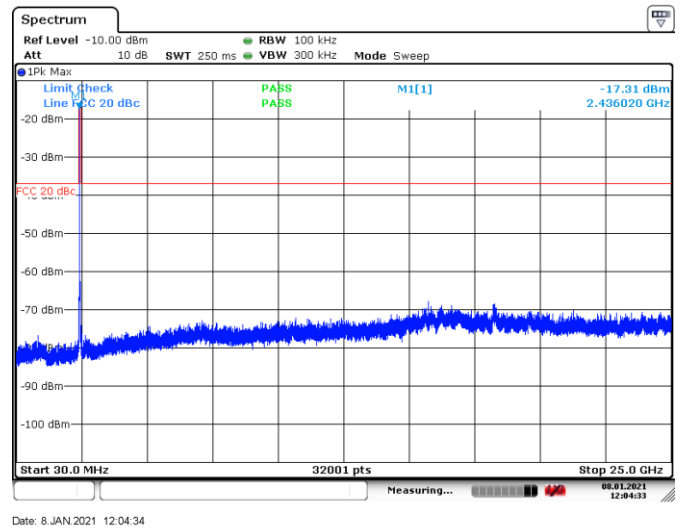
Figure 8.7-8: Conducted spurious emissions, tx on mid channel, Tx on 802.11b
