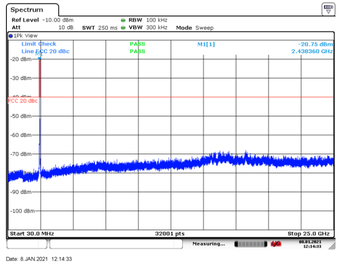
Figure 8.7-14: Conducted spurious emissions, tx on mid channel, Tx on 802.11n
