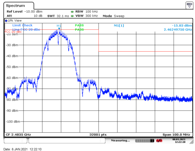
Figure 8.7-2: Conducted Band edge spurious emissions at 2483.5 MHz, Tx on 802.11b
