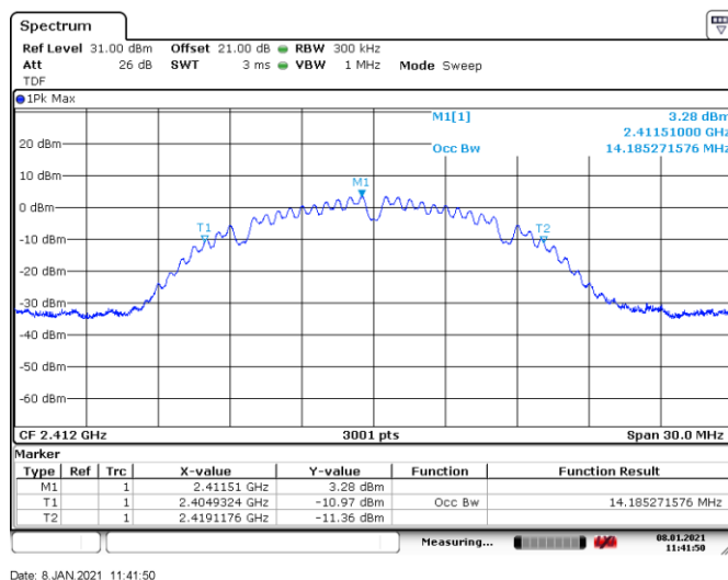
Figure 8.5-4: 99% occupied bandwidth on 802.11b, sample plot
