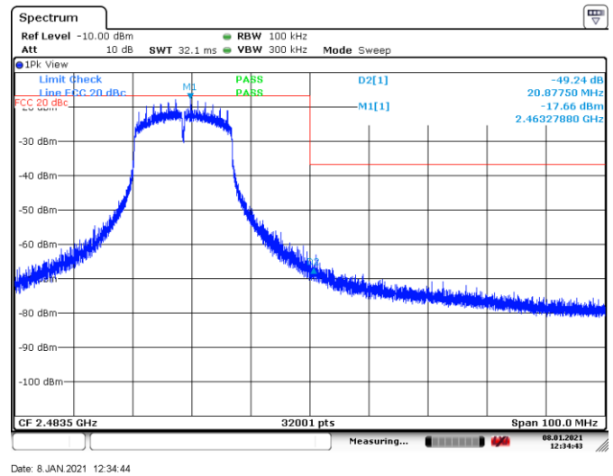
Figure 8.7-6: Conducted Band edge spurious emissions at 2483.5 MHz, Tx on 802.11n
