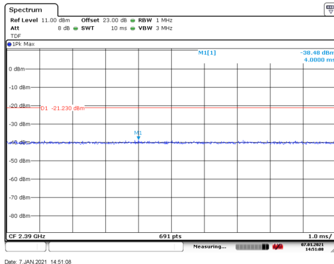
Figure 8.7-16: Conducted spurious emissions on 2390 MHz, peak, Tx on 802.11b
