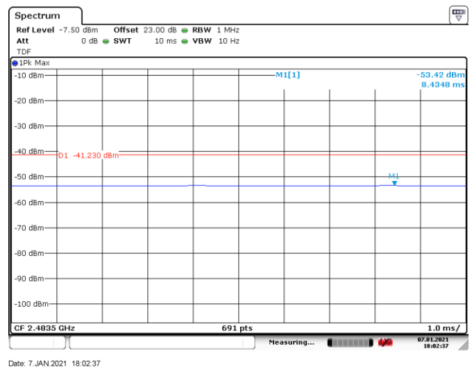
Figure 8.7-19: Conducted spurious emissions on 2483.5MHz, average, Tx on 802.11b
