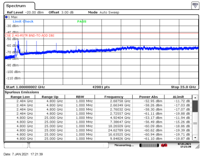
Figure 8.7-33: Conducted spurious emissions above 1 GHz within restricted bands, Tx on high channel of 802.11b
