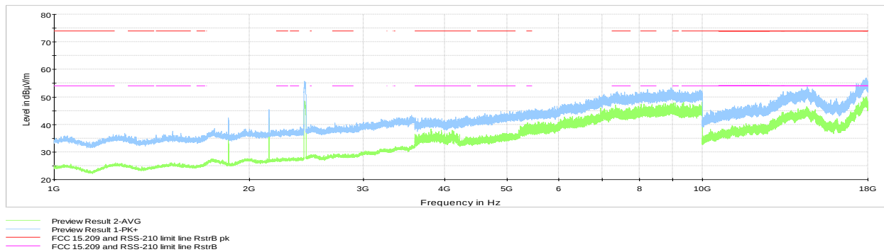
Figure 8.7-50: Cabinet radiated Spurious emissions 1to18 GHz, Tx @ mid channel
