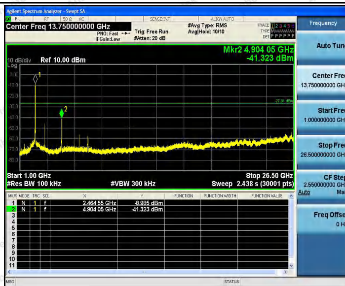
11N40_Ant3_2452_0~Reference
