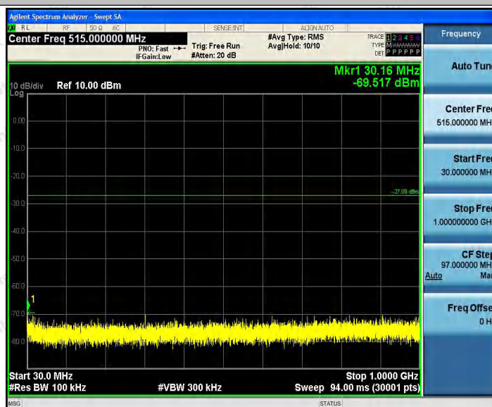
11N40_Ant3_2452_30~1000
