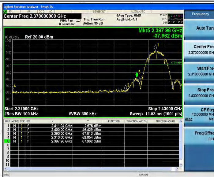
11B_Ant3_Low_2412
