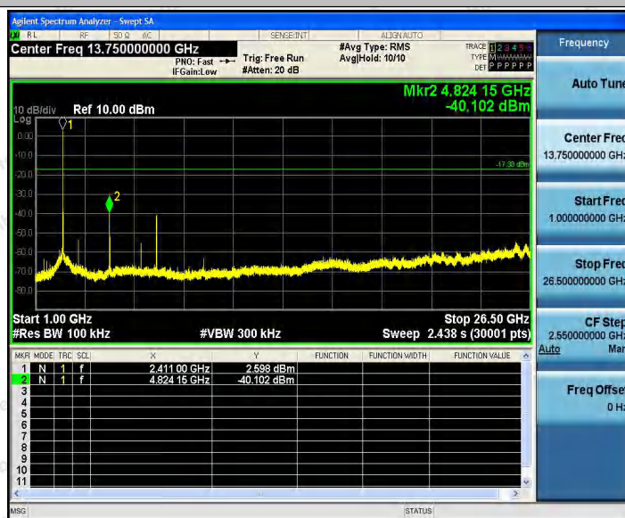
11B_Ant3_2412_0~Reference
