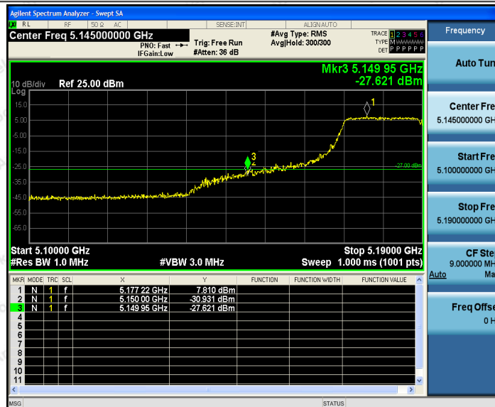
11AC40SISO_Ant2_Low_5190
