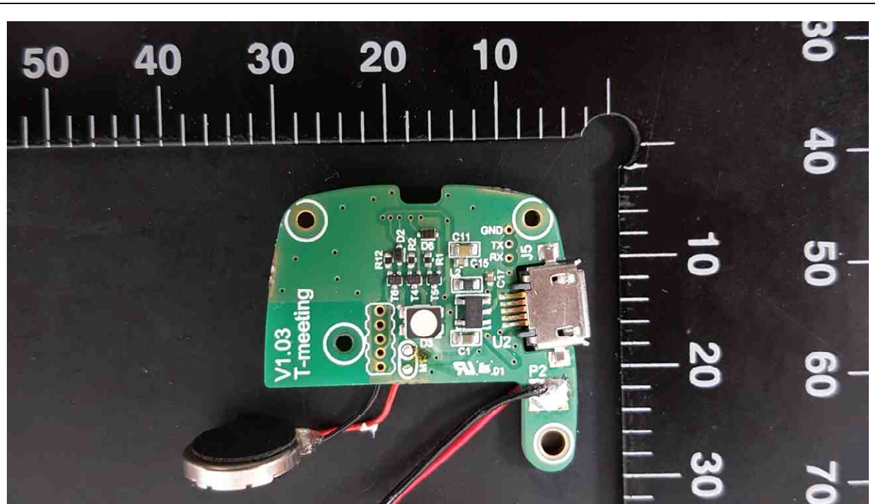
Main Board_Rear
