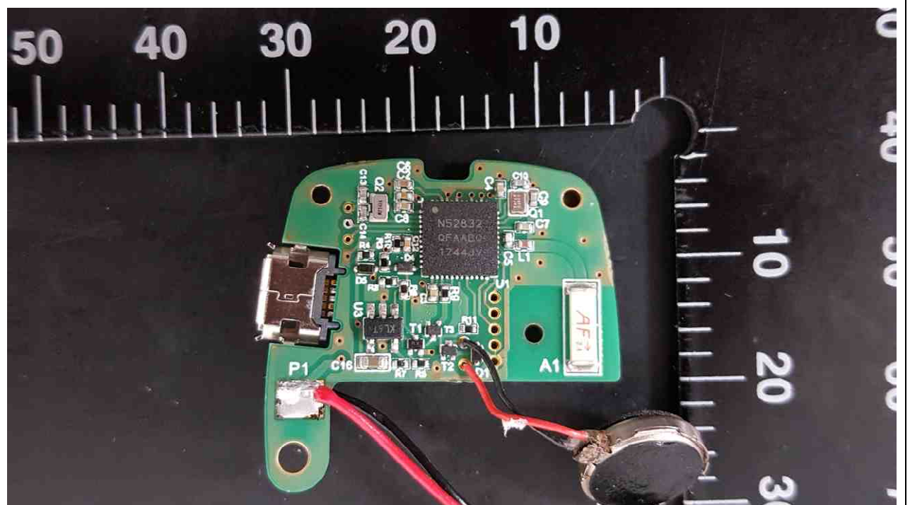
Main Board Front
