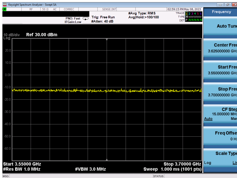
Plot 34. Conducted Measurement – No RF transmission in entire band at anytime (WINNF.FT.C.SCS.5)
