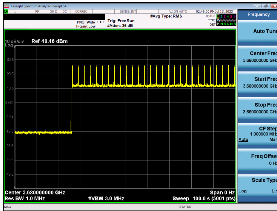
Plot 11. Conducted Measurement - RF transmission after SAS heartbeat response (WINNF.FT.D.HBT.2)
