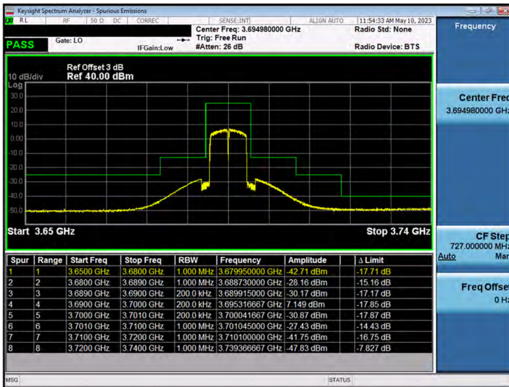
Plot 7.199. Conducted Band Edge Plot (10MHz, QPSK, High Channel, Ch.B)
