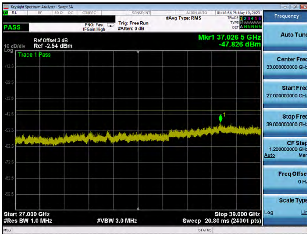
Plot 7.180. Conducted Spurious Plot (10MHz QPSK, Mid Channel – Ch.B)
