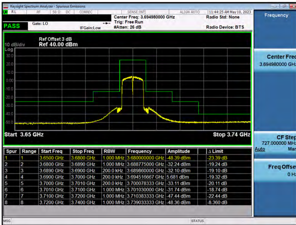
Plot 7.187. Conducted Band Edge Plot (10MHz, QPSK, High Channel, Ch.A)
