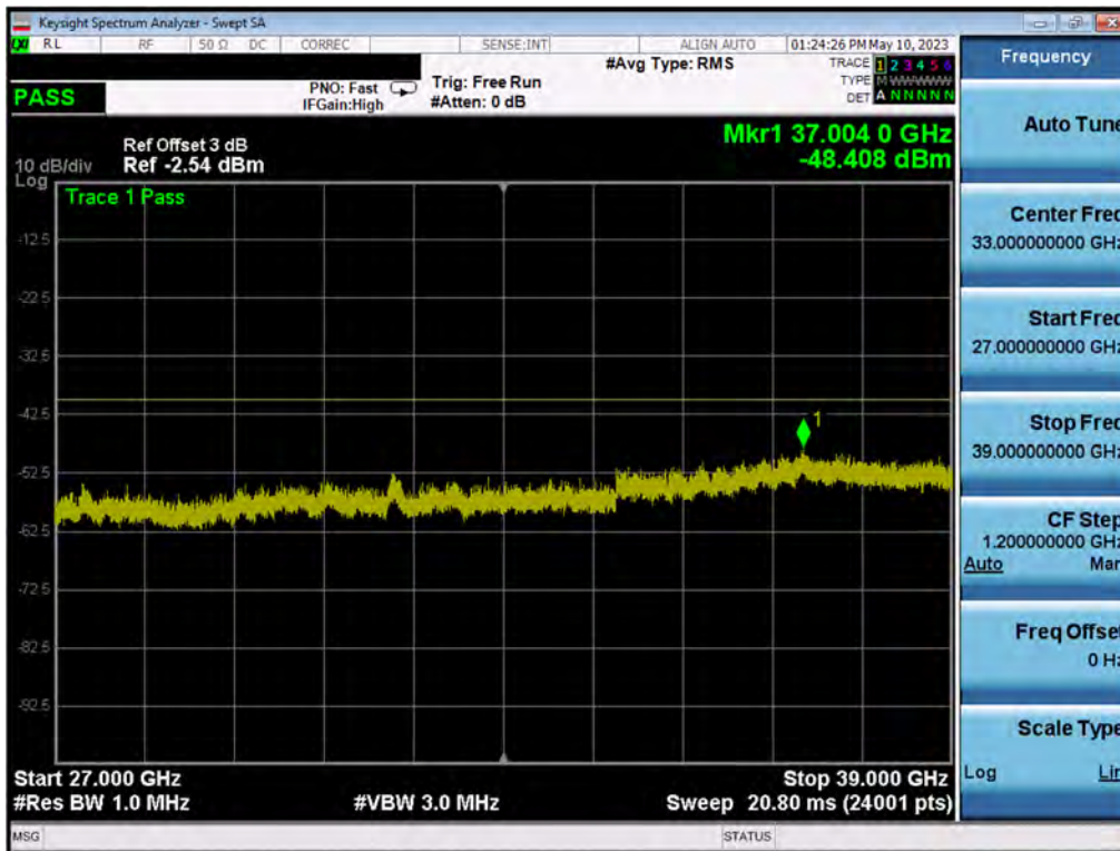
Plot 7.184. Conducted Spurious Plot (10MHz QPSK, High Channel – Ch.B)
