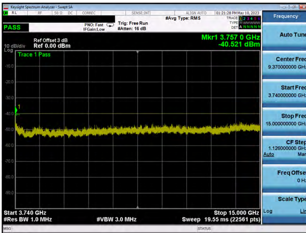
Plot 7.170. Conducted Spurious Plot (10MHz QPSK, High Channel – Ch.A)
