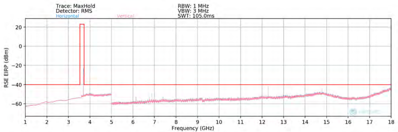
Plot 7.212. Radiated Spurious Plot 1-18GHz – High Channel
