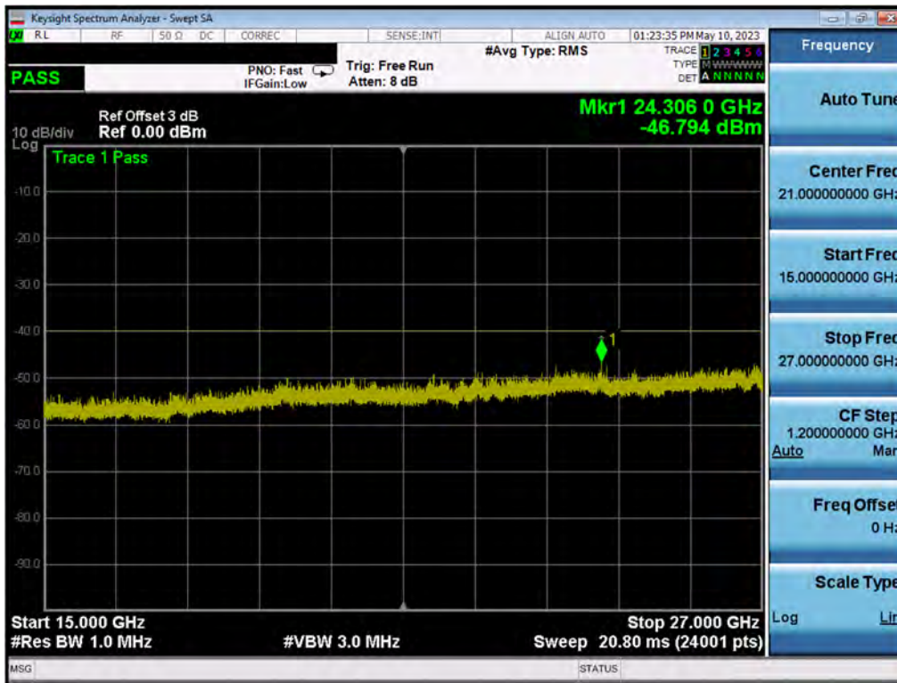
Plot 7.183. Conducted Spurious Plot (10MHz QPSK, High Channel – Ch.B)
