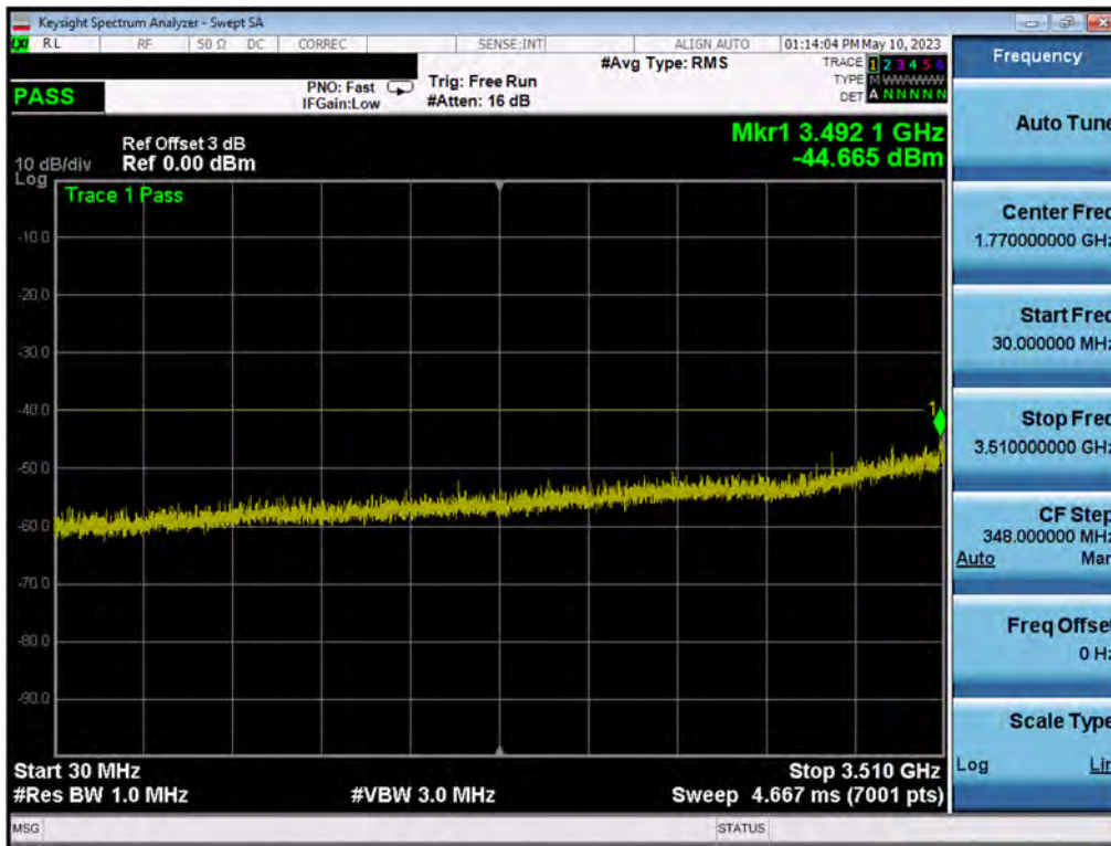
Plot 7.173. Conducted Spurious Plot (10MHz QPSK, Low Channel – Ch.B)
