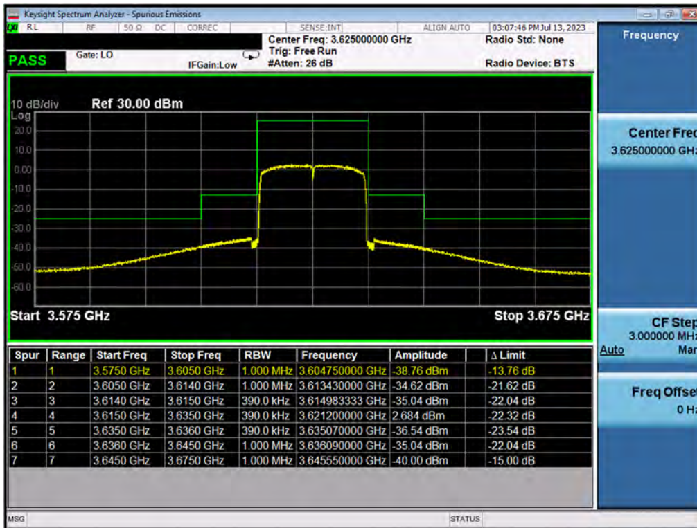
Plot 7.201. Conducted Band Edge Plot (20MHz, QPSK, Mid Channel, Ch.B)
