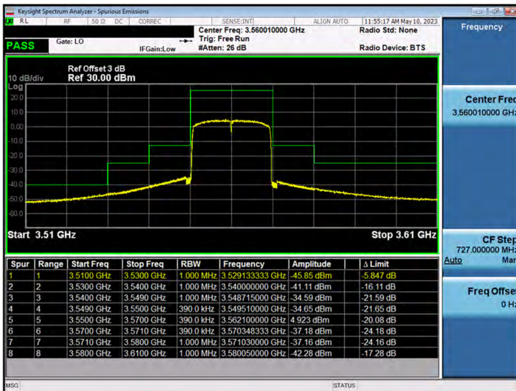
Plot 7.200. Conducted Band Edge Plot (20MHz, QPSK, Low Channel, Ch.B)
