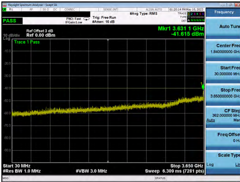
Plot 7.169. Conducted Spurious Plot (10MHz QPSK, High Channel – Ch.A)
