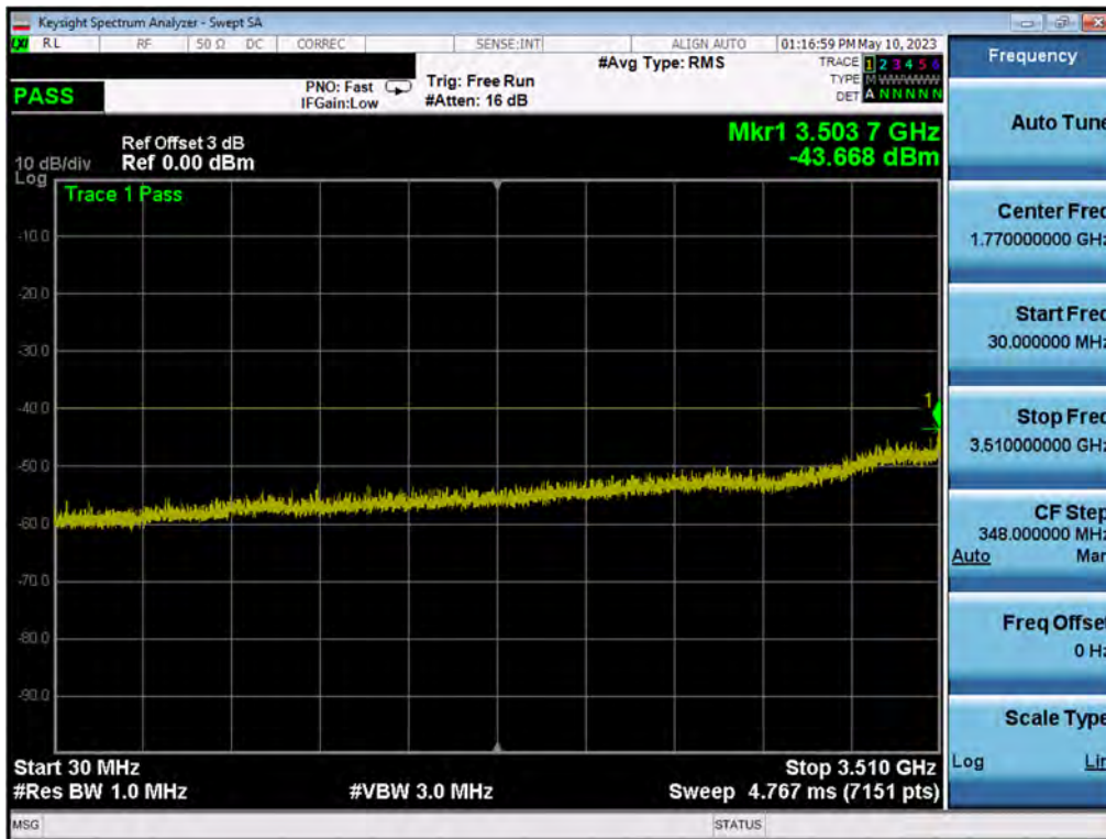
Plot 7.177. Conducted Spurious Plot (10MHz QPSK, Mid Channel – Ch.B)
