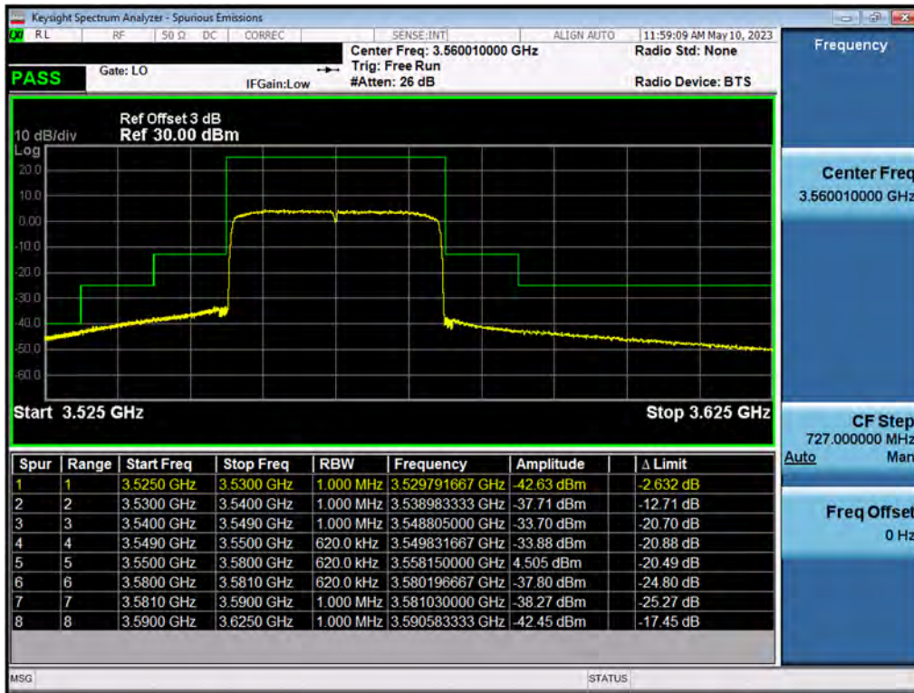
Plot 7.203. Conducted Band Edge Plot (30MHz, QPSK, Low Channel, Ch.B)
