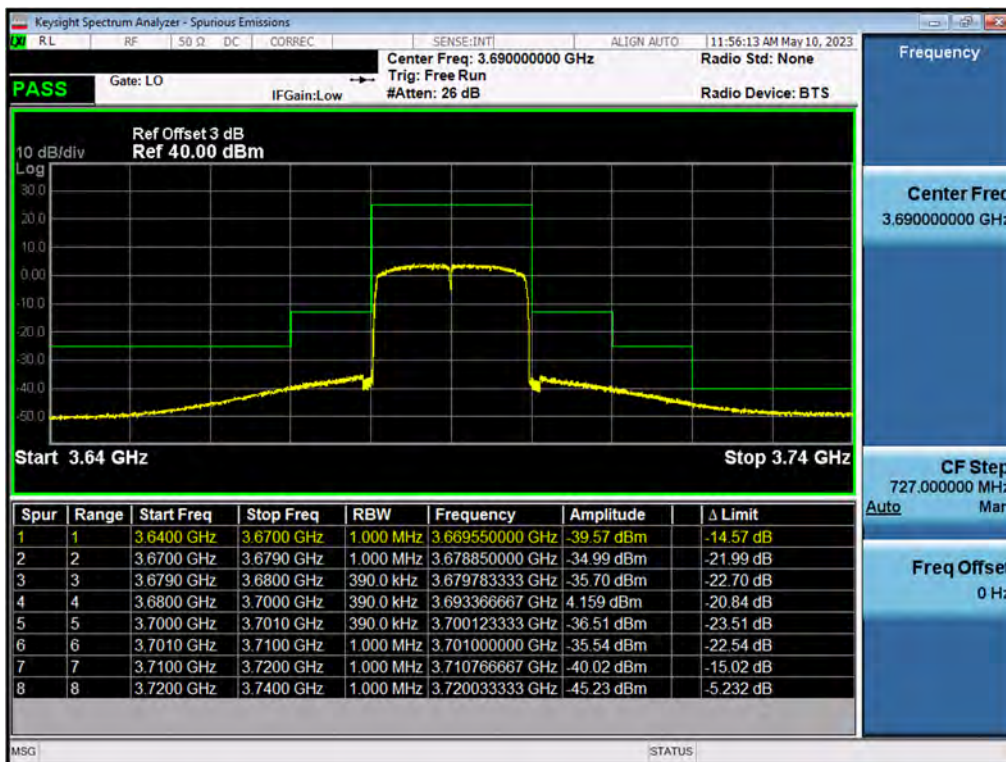
Plot 7.202. Conducted Band Edge Plot (20MHz, QPSK, High Channel, Ch.B)
