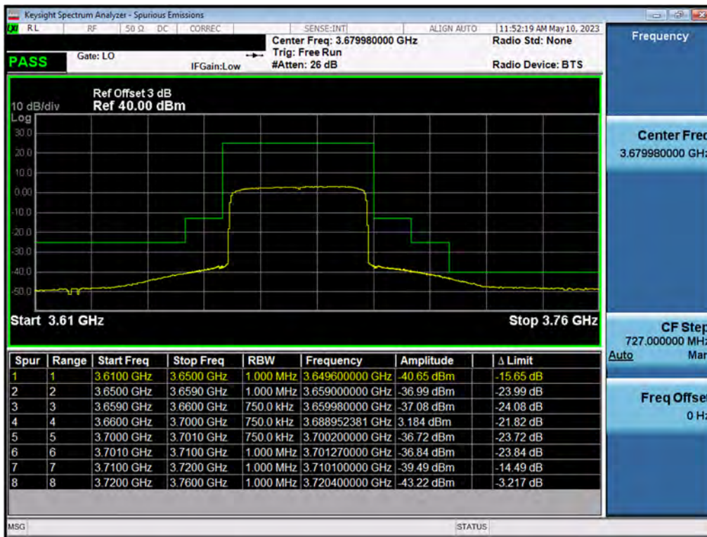
Plot 7.196. Conducted Band Edge Plot (40MHz, QPSK, High Channel, Ch.A)
