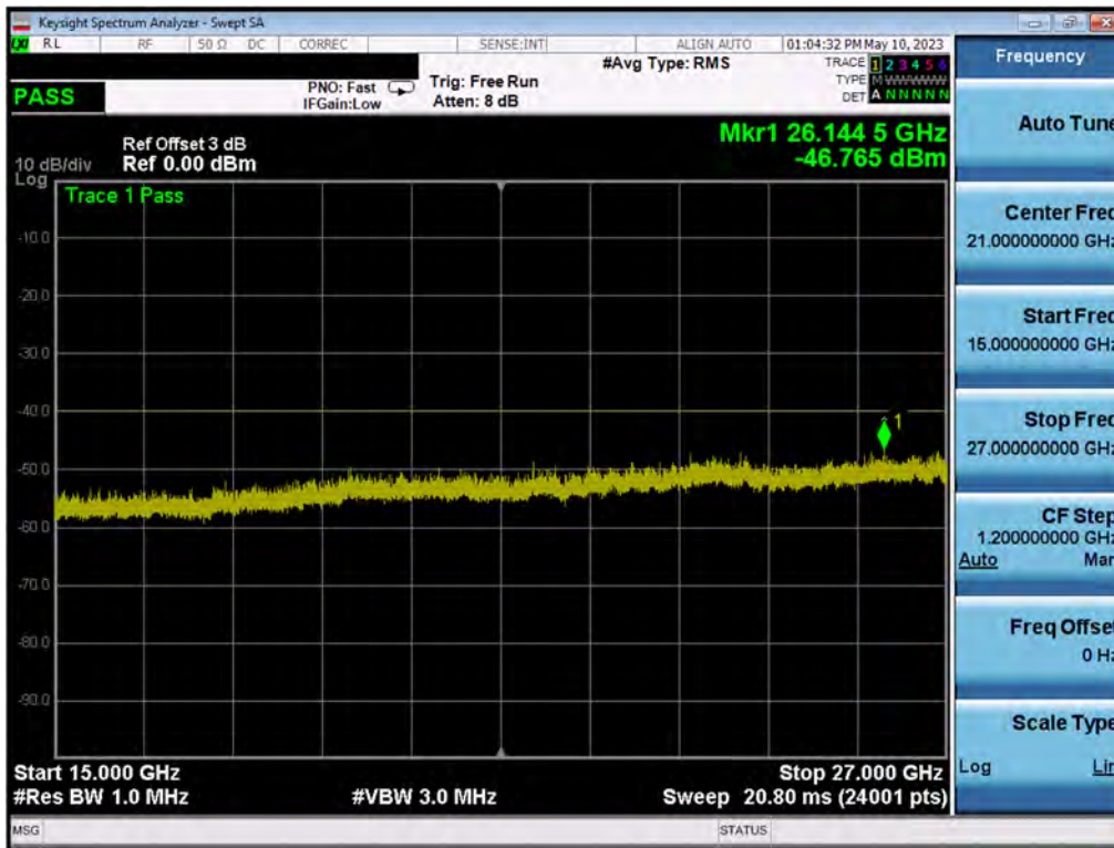
Plot 7.167. Conducted Spurious Plot (10MHz QPSK, Mid Channel – Ch.A)
