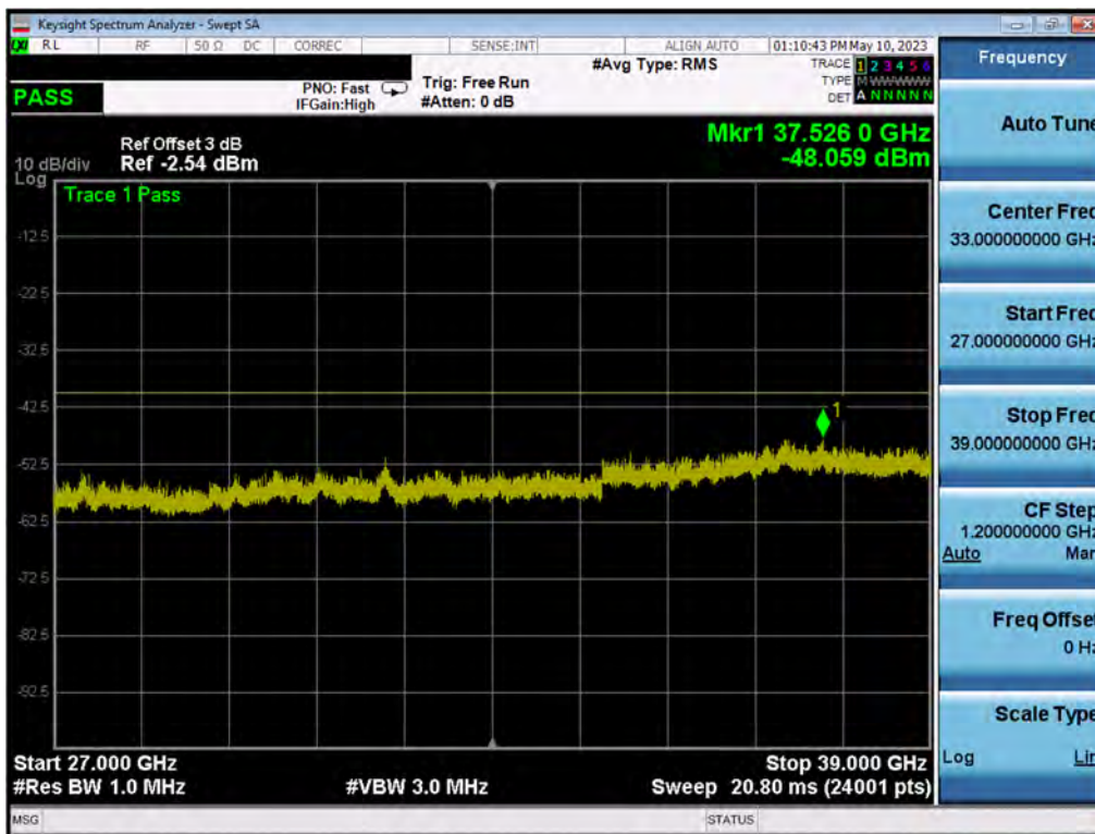
Plot 7.172. Conducted Spurious Plot (10MHz QPSK, High Channel – Ch.A)
