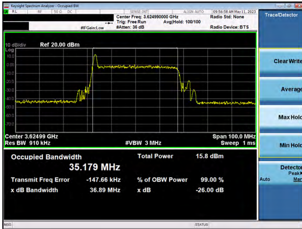
Plot 7.35. Occupied Bandwidth Plot (40MHz 64-QAM – Ch.A)
