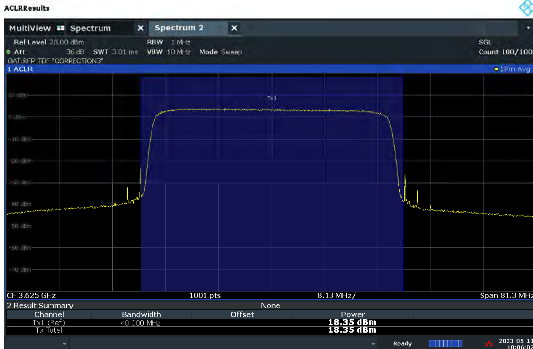
Plot 7.13 – Conducted Power Measurement – 40MHz BW, Mid Channel, QPSK – Ch.A
