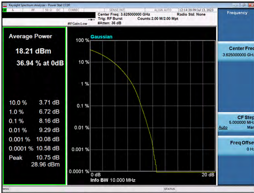
Plot 7.141. Peak to Average Power Ratio Plot (10MHz, QPSK – Mid Channel) – Ch.A
