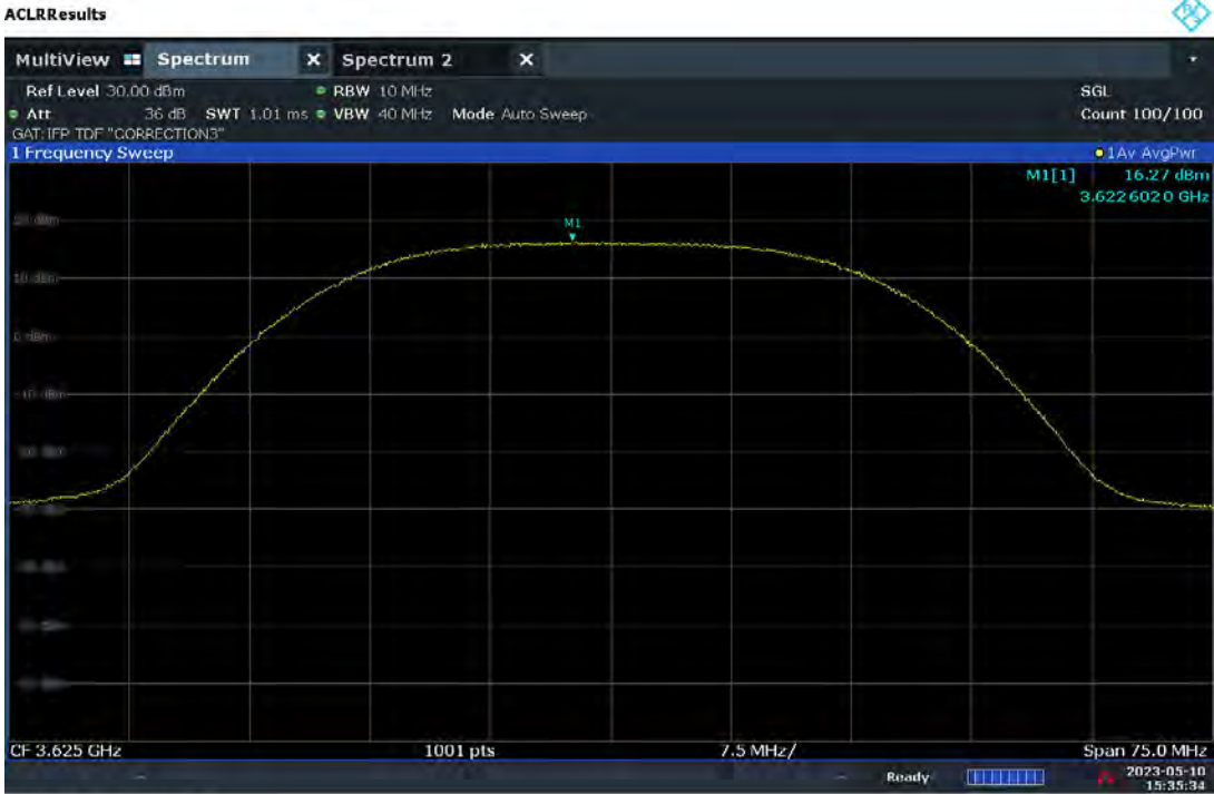
Plot 7.91. Conducted Power / 10MHz (30MHz 64QAM, Mid Channel – Ch.B)
