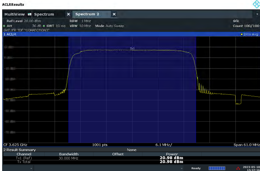
Plot 7.28 – Conducted Power Measurement – 30MHz BW, Mid Channel, 256QAM – Ch.B
