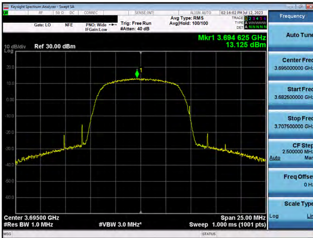
Plot 7.114. Power Spectral Density (10MHz 16QAM, High Channel – Ch.B)
