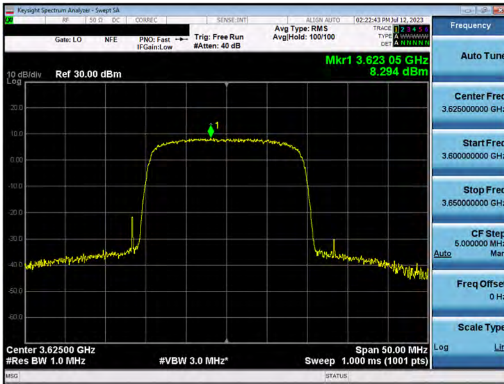
Plot 7.119. Power Spectral Density (20MHz 64QAM, Mid Channel – Ch.B)
