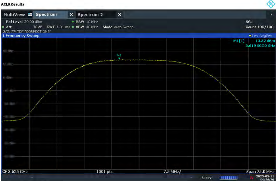
Plot 7.76. Conducted Power / 10MHz (30MHz 256QAM, Mid Channel – Ch.A)
