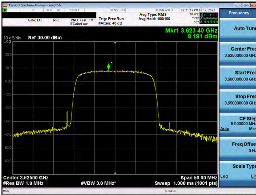
Plot 7.117. Power Spectral Density (20MHz QPSK, Mid Channel – Ch.B)
