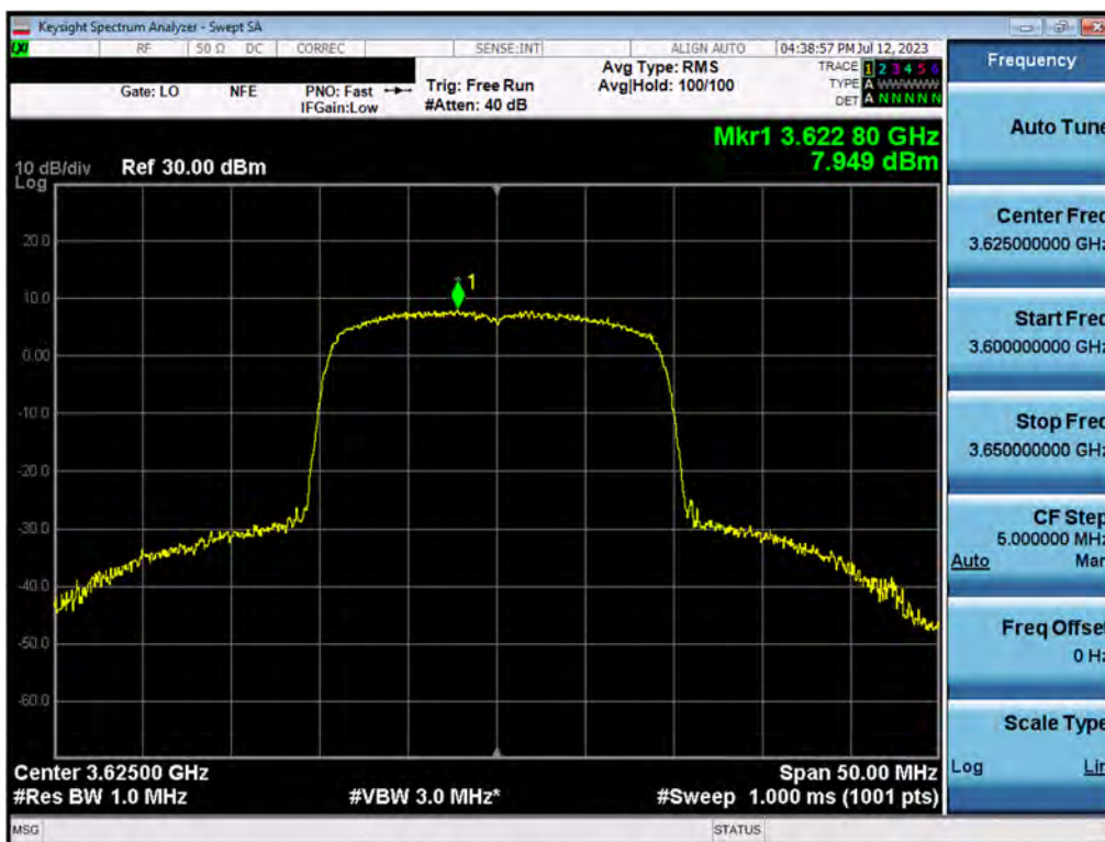
Plot 7.104. Power Spectral Density (20MHz 256QAM, Mid Channel – Ch.A)
