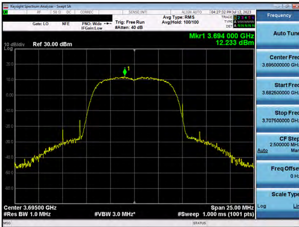
Plot 7.98. Power Spectral Density (10MHz 16QAM, High Channel – Ch.A)
