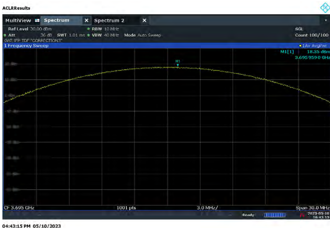
Plot 7.68. Conducted Power / 10MHz (10MHz 256QAM, High Channel – Ch.A)
