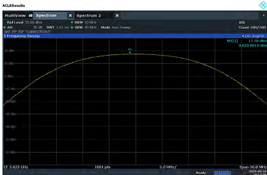
Plot 7.88. Conducted Power / 10MHz (20MHz 256QAM, Mid Channel – Ch.B)
