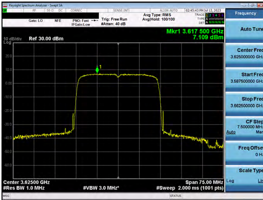
Plot 7.123. Power Spectral Density (30MHz 64QAM, Mid Channel – Ch.B)
