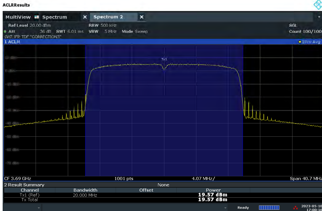
Plot 7.7 – Conducted Power Measurement – 20MHz BW, High Channel, 64QAM – Ch.A
