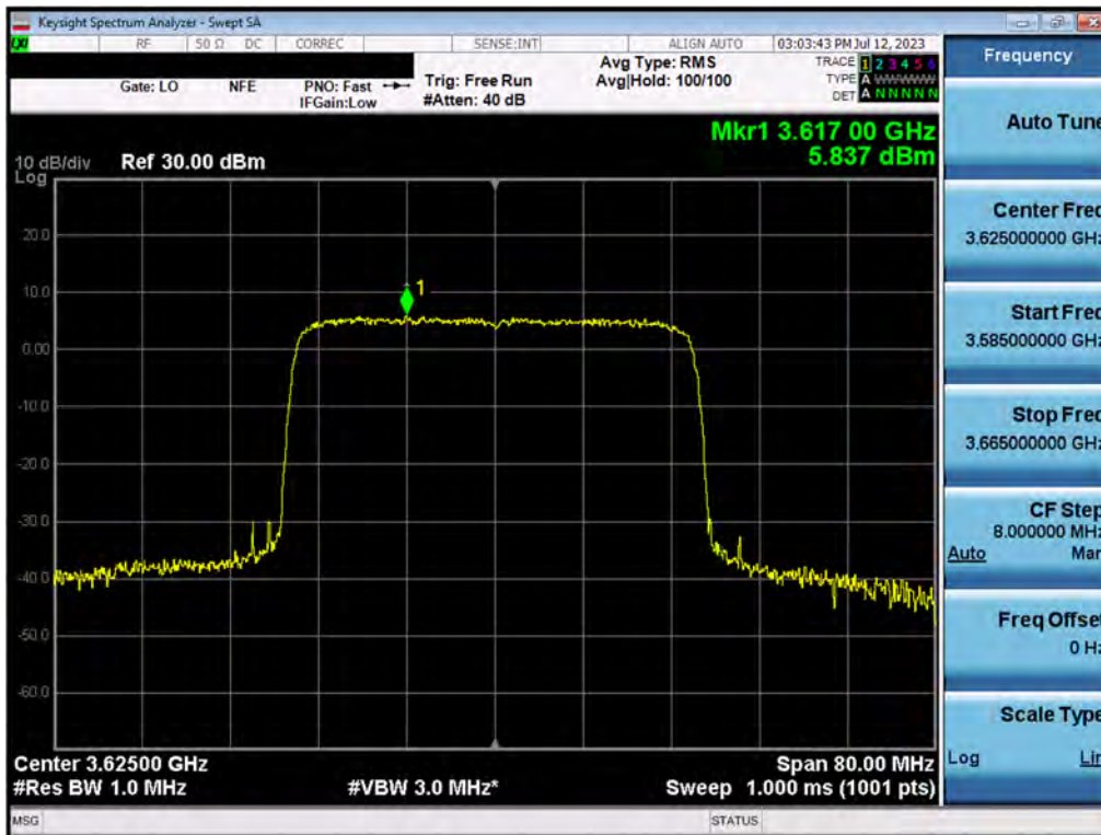
Plot 7.125. Power Spectral Density (40MHz QPSK, Mid Channel – Ch.B)
