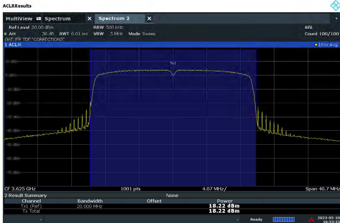
Plot 7.6 – Conducted Power Measurement – 20MHz BW, Mid Channel, 16QAM – Ch.A
