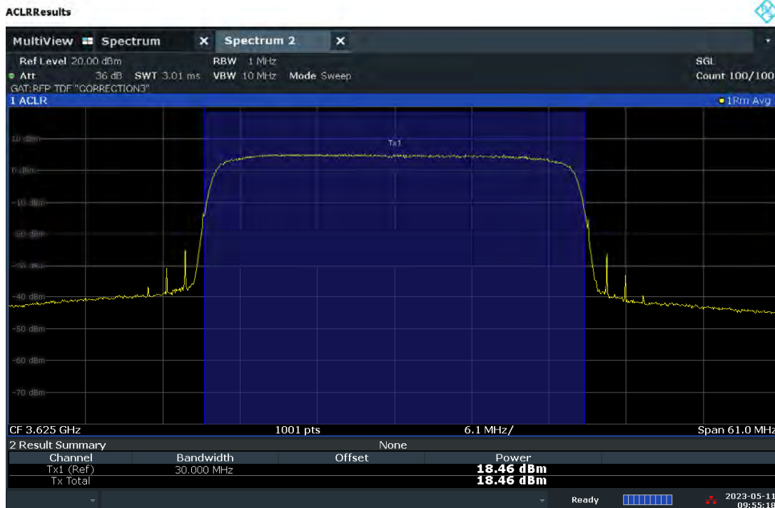
Plot 7.11 – Conducted Power Measurement – 30MHz BW, Mid Channel, 64QAM – Ch.A
