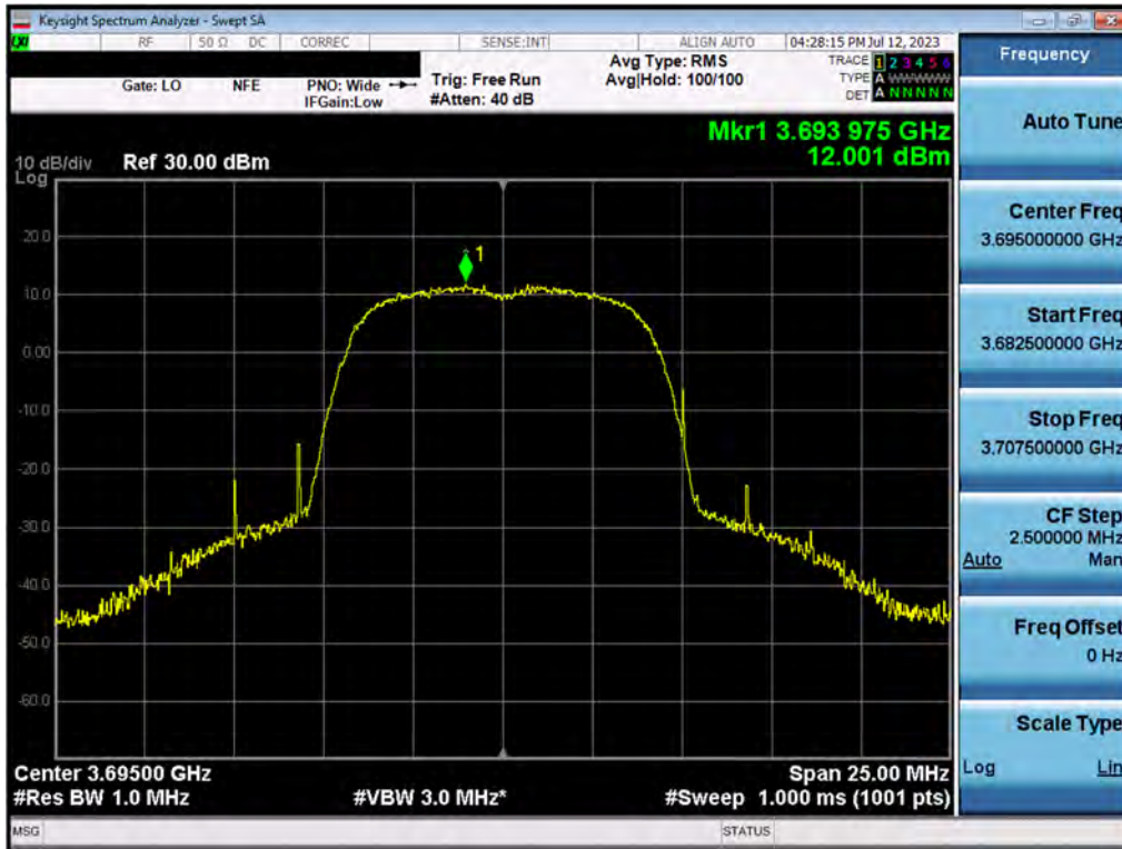
Plot 7.99. Power Spectral Density (10MHz 64QAM, High Channel – Ch.A)
