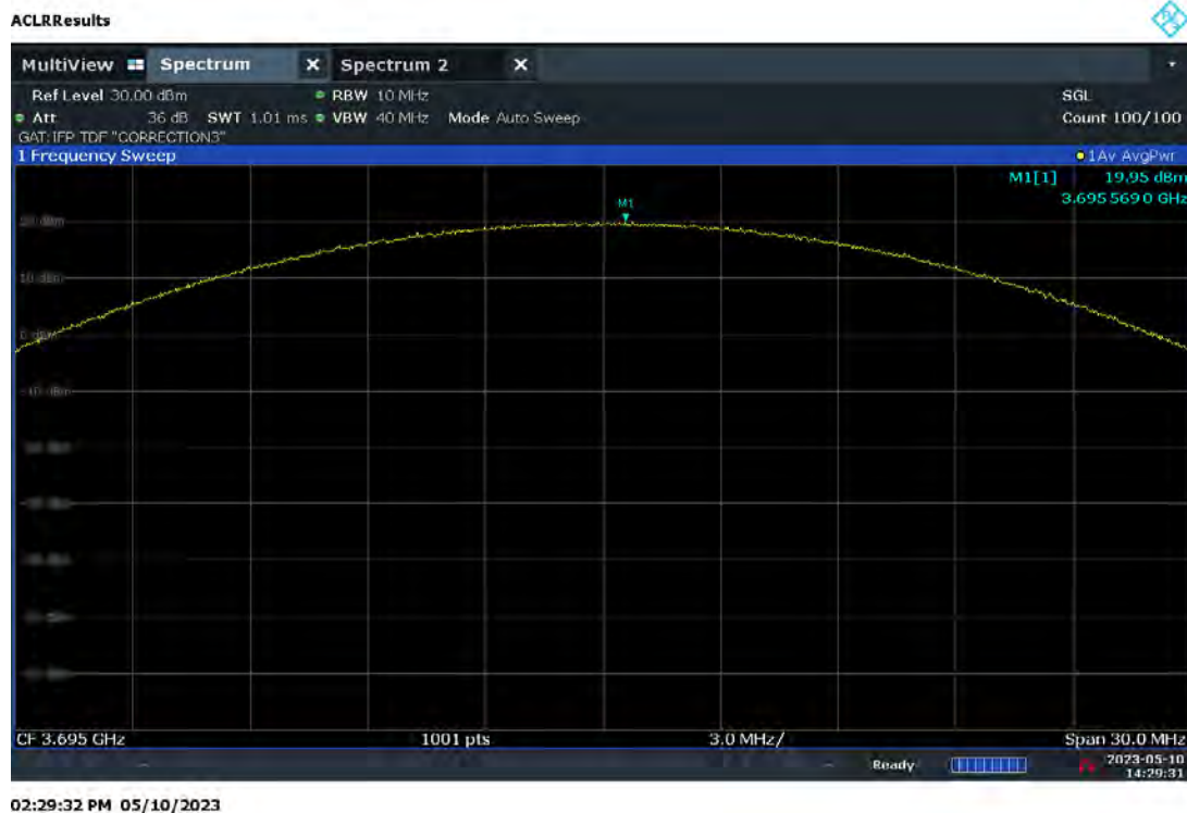
Plot 7.83. Conducted Power / 10MHz (10MHz 64QAM, High Channel – Ch.B)
