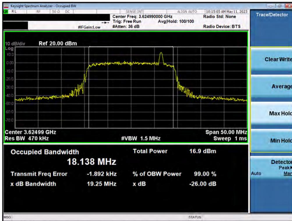
Plot 7.58. Occupied Bandwidth Plot (20MHz 16-QAM – Ch.B)
