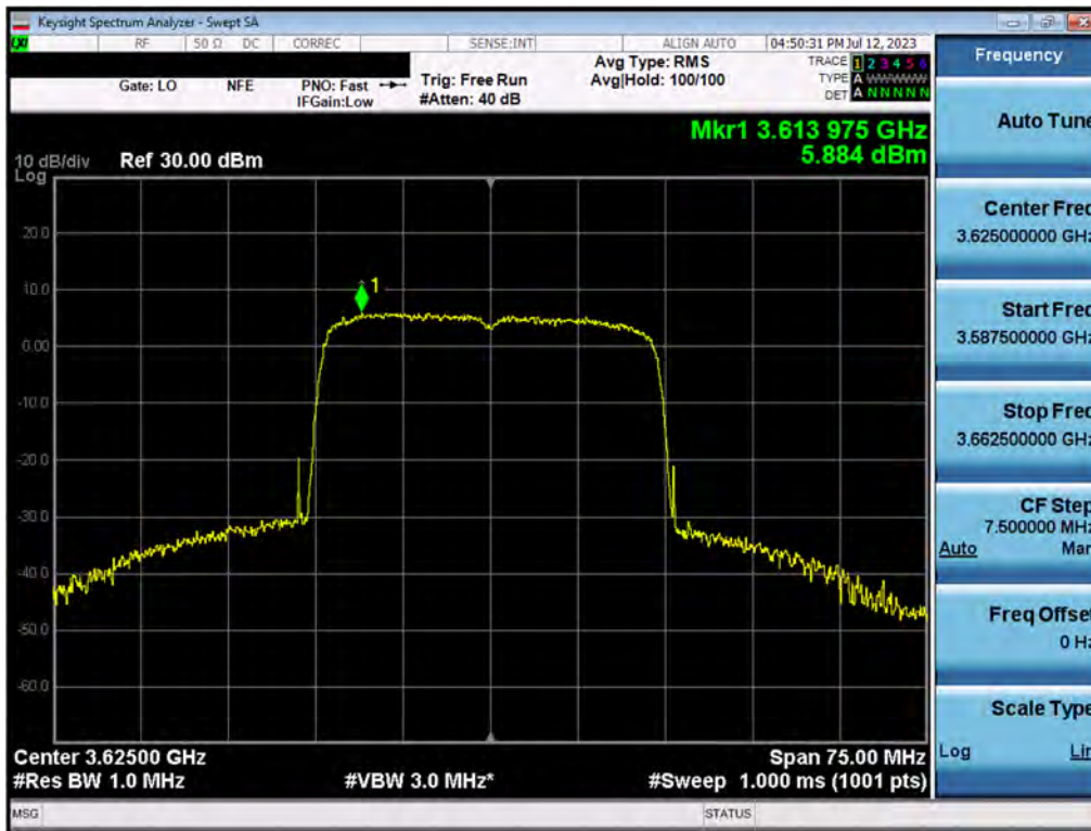
Plot 7.107. Power Spectral Density (30MHz 64QAM, Mid Channel – Ch.A)
