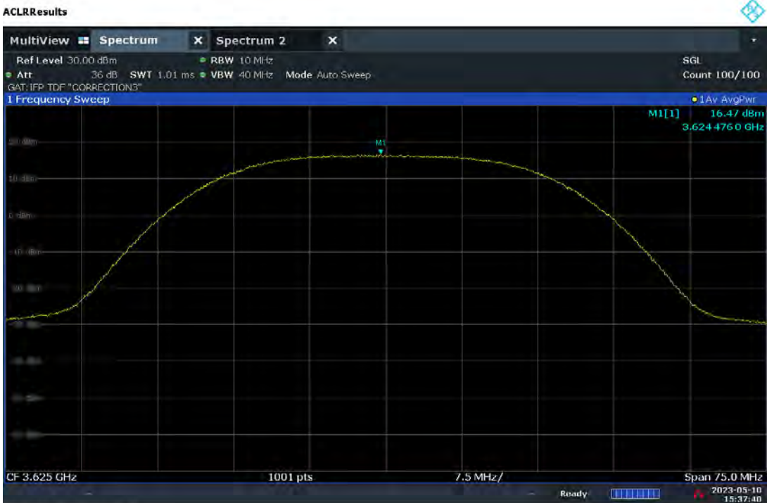
Plot 7.92. Conducted Power / 10MHz (30MHz 256QAM, Mid Channel – Ch.B)
