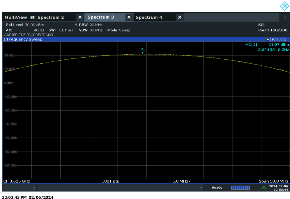
Plot 7.21 – Conducted Power Measurement – 20MHz BW, Mid Channel, QPSK – ANT2
