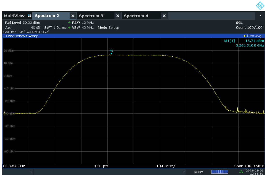
Plot 7.95. Conducted Power / 10MHz (40MHz 64QAM, Low Channel – ANT2)
