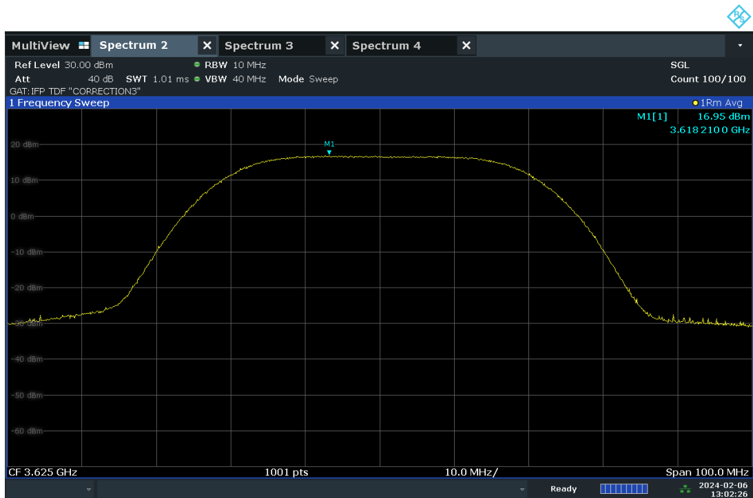
Plot 7.96. Conducted Power / 10MHz (40MHz 256QAM, Mid Channel – ANT2)
