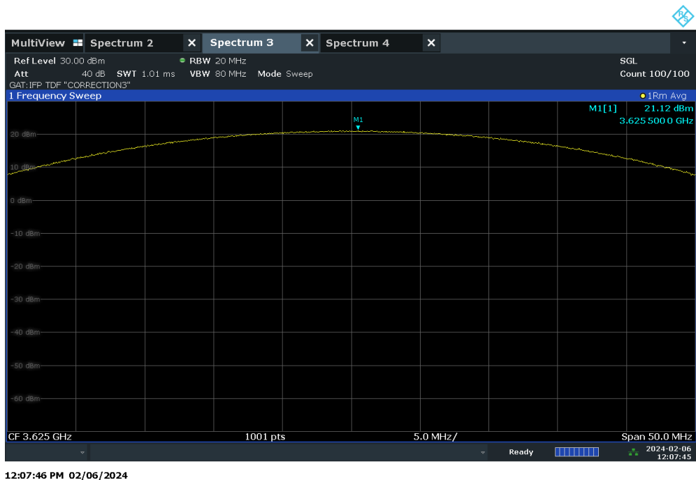
Plot 7.24 – Conducted Power Measurement – 20MHz BW, Mid Channel, 256QAM – ANT2
