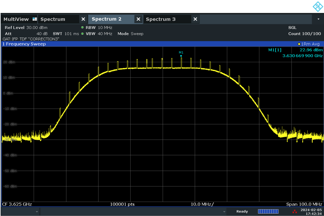
Plot 7.80. Conducted Power / 10MHz (40MHz 256QAM, Mid Channel – ANT1)
