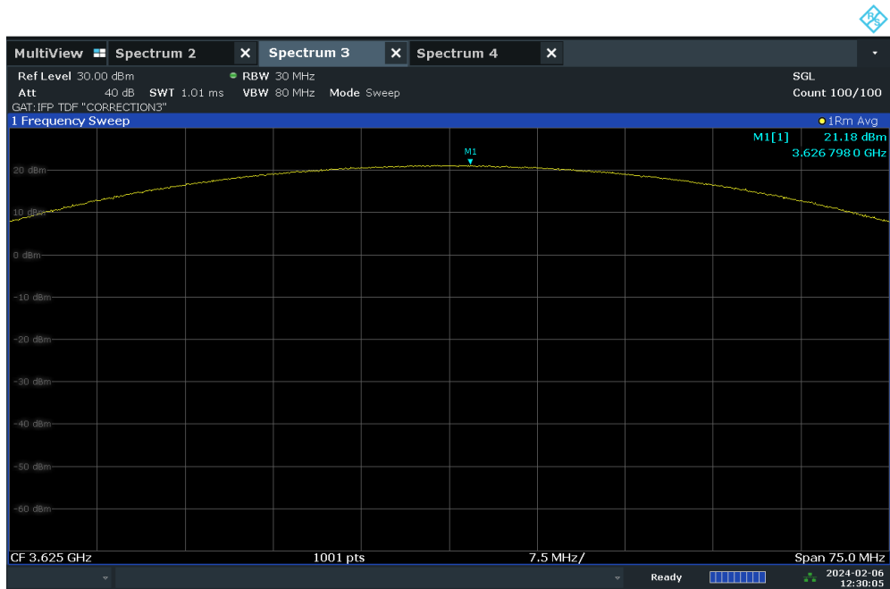
Plot 7.28 – Conducted Power Measurement – 30MHz BW, Mid Channel, 256QAM – ANT2
