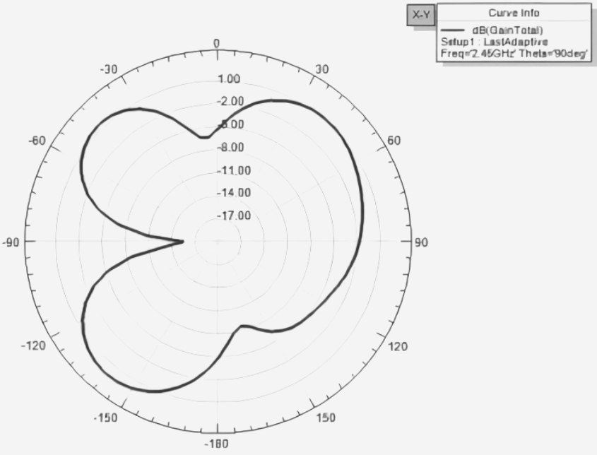
Radiation Pattern 2
