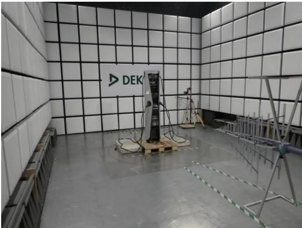
Figure B2: Radiated Emission Setup OM#1
