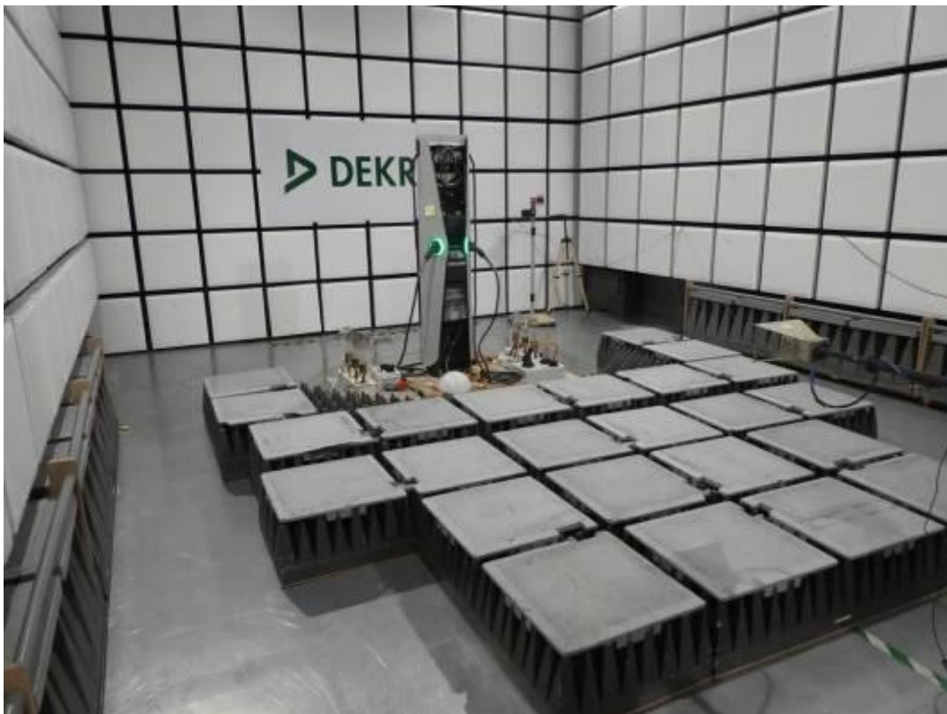
Figure B4: High range Radiated Emission Test Setup
