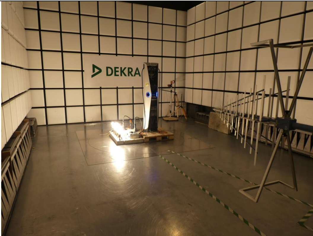
Figure B3: Radiated Emission Setup OM#2
