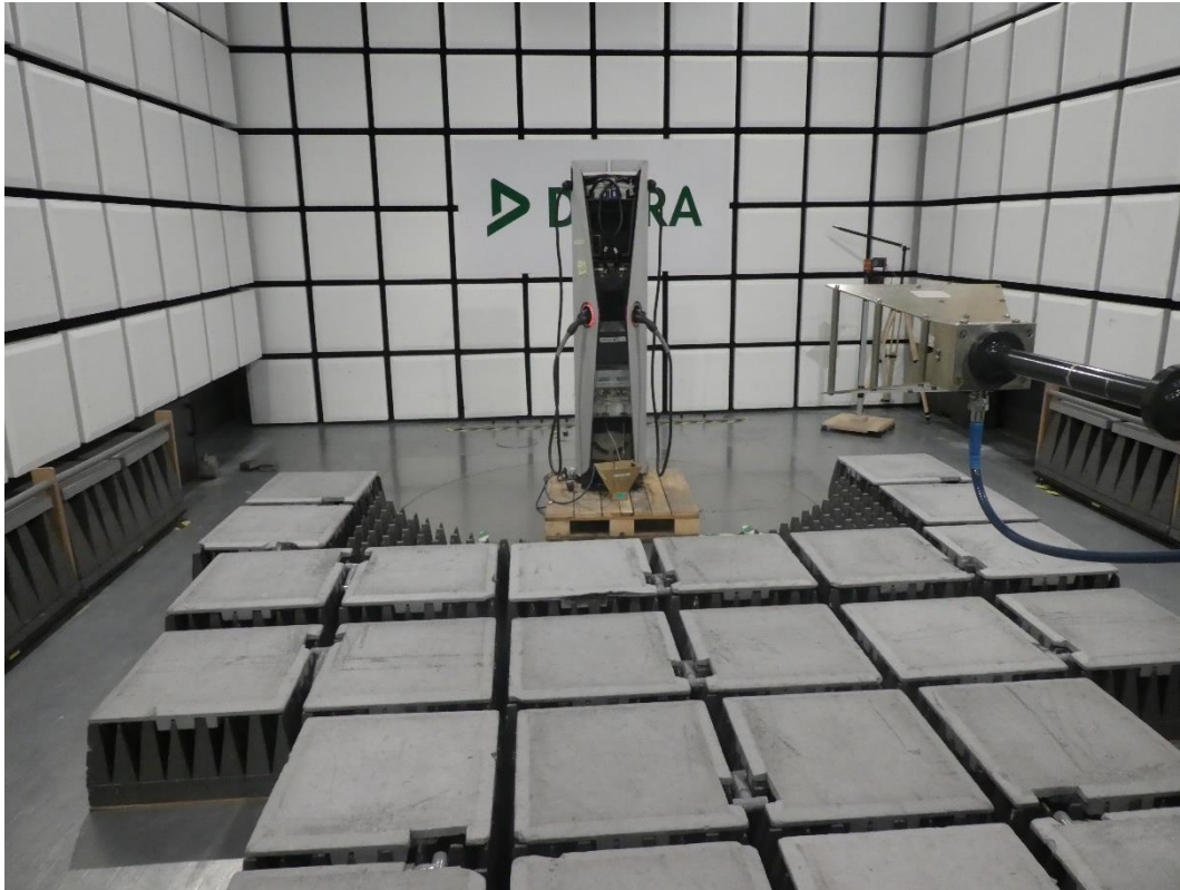
Figure B3: Radiated Emission above 1 GHz.
