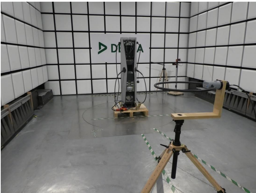
Figure B2: Radiated Emission 9 kHz – 30 MHz
