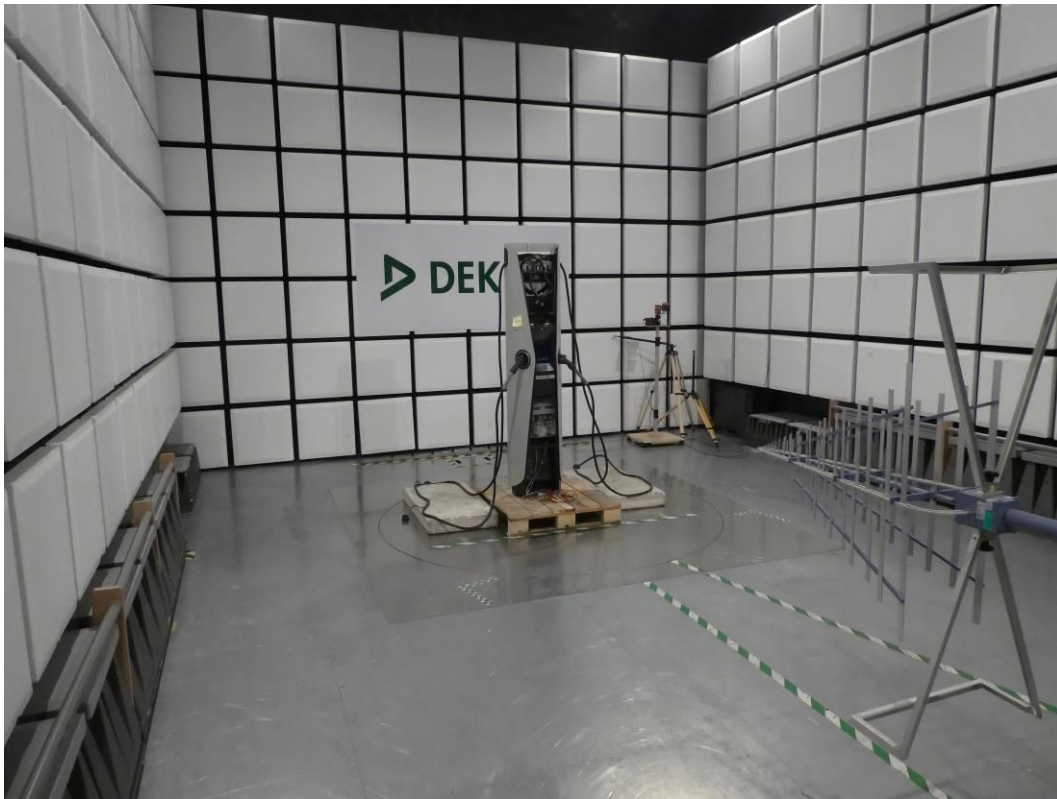
Figure B1: Radiated Emissions 30 MHz – 1GHz
