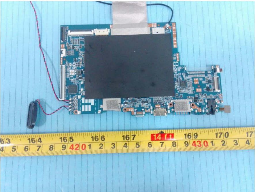
EUT –Tablet Main Board Top View 1
