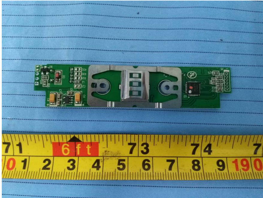
EUT – External Module MSR Board Bottom View
