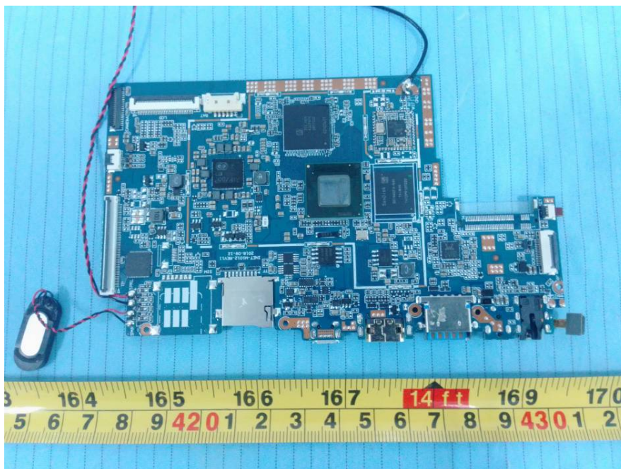
EUT –Tablet Main Board Top Shielding off View
