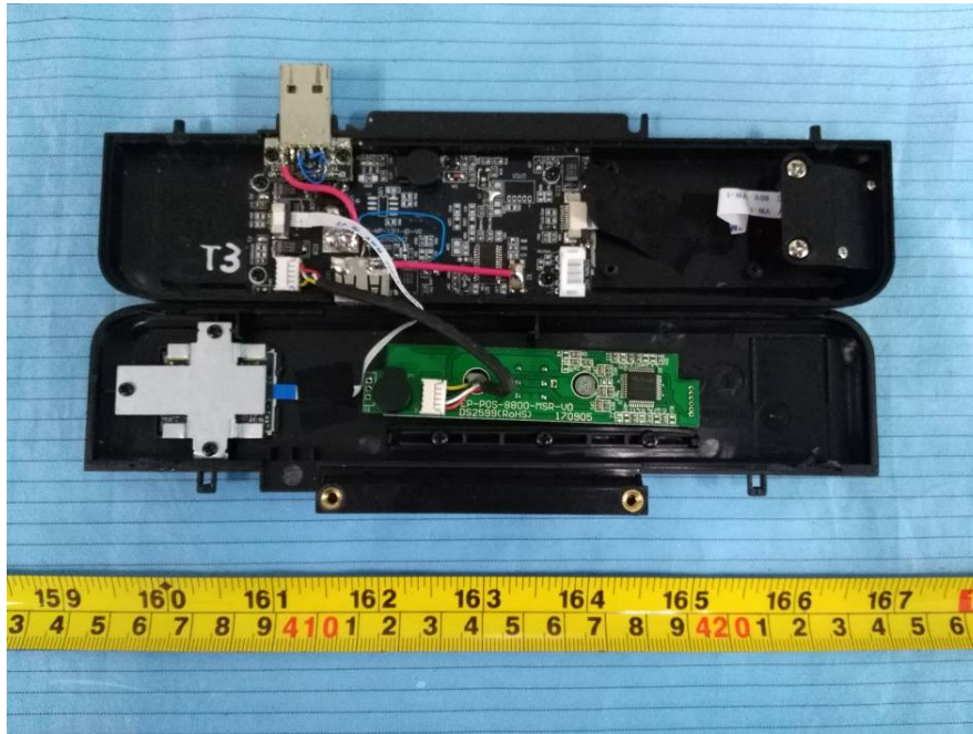
EUT – External Module Cover off View
