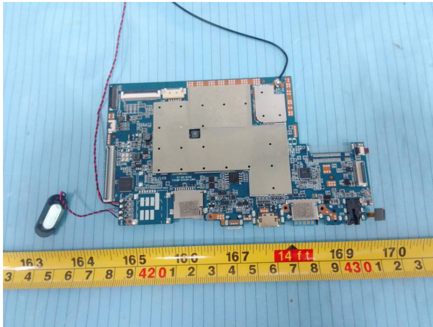
EUT –Tablet Main Board Top View 2
