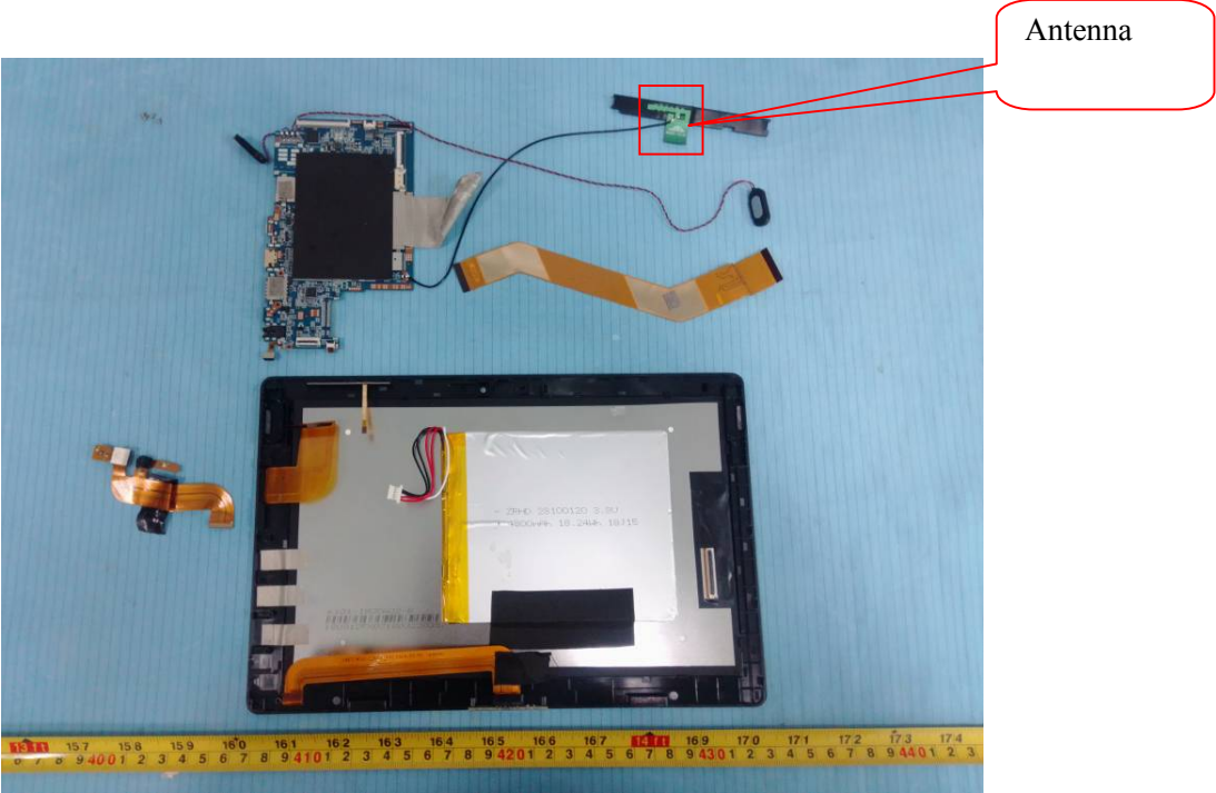
EUT –Tablet Cover off View 2
