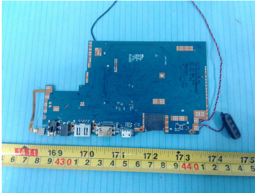
EUT –Tablet Main Board Bottom View
