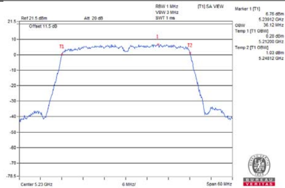
802.11n (HT40) / Chain 3 / CH 46
