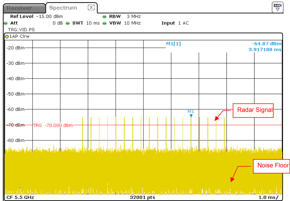
Radar Signal 3
