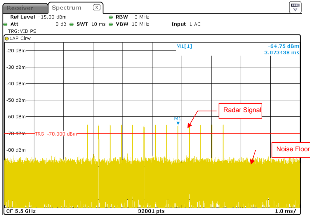
Radar Signal 4
