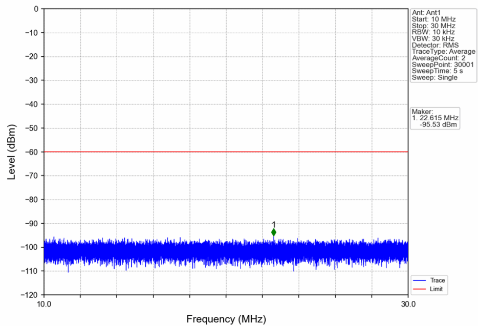
n48_30kHz_SISO_NTNV_10MHz_CP-OFDM QPSK_3624.99MHz_Edge_1RB_Left
