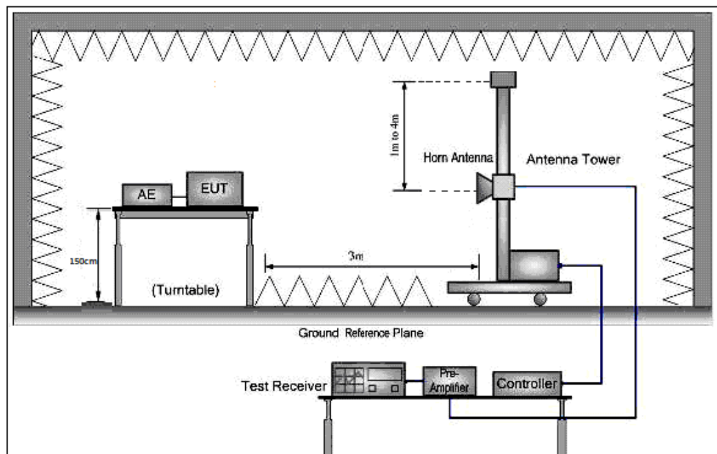
Above 1GHz
