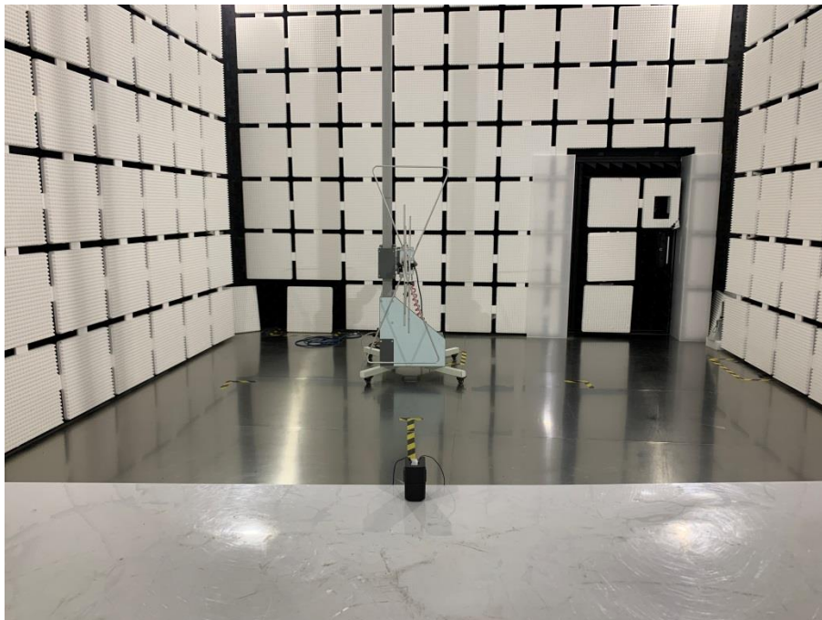
Radiated Measurement
