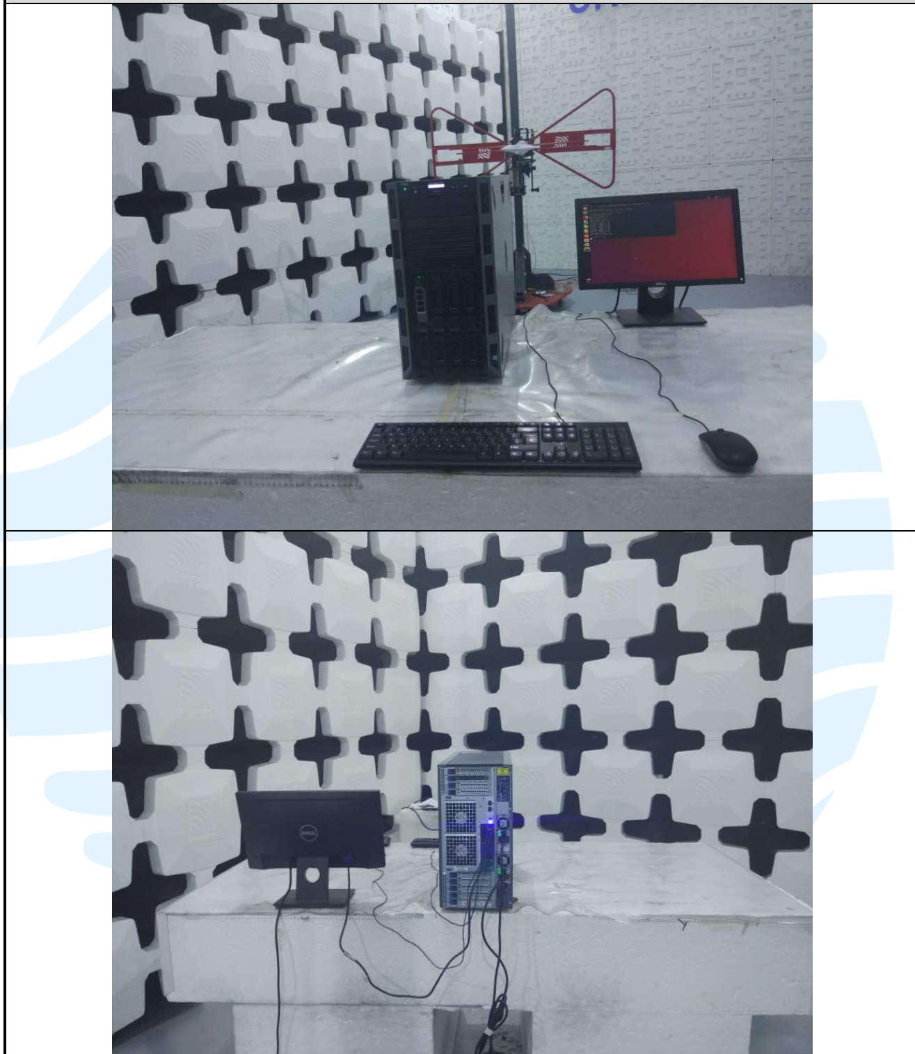
Radiated emission Test Setup-1 (30 MHz~1 GHz)
