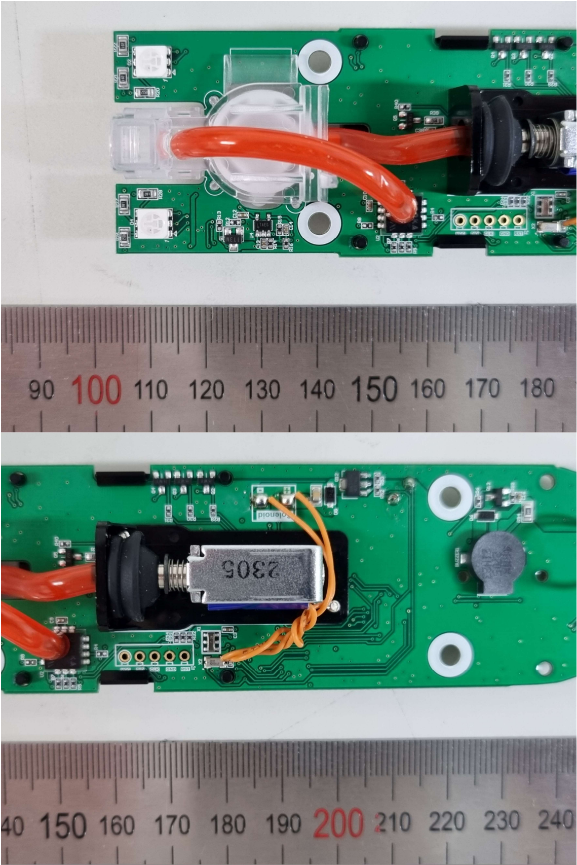
Main Board (Rear, Scale up)
