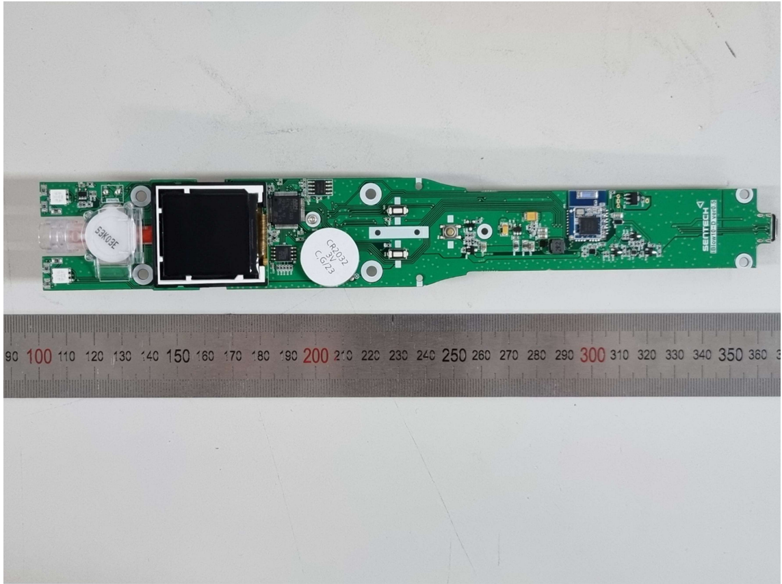
Main Board(Front)
