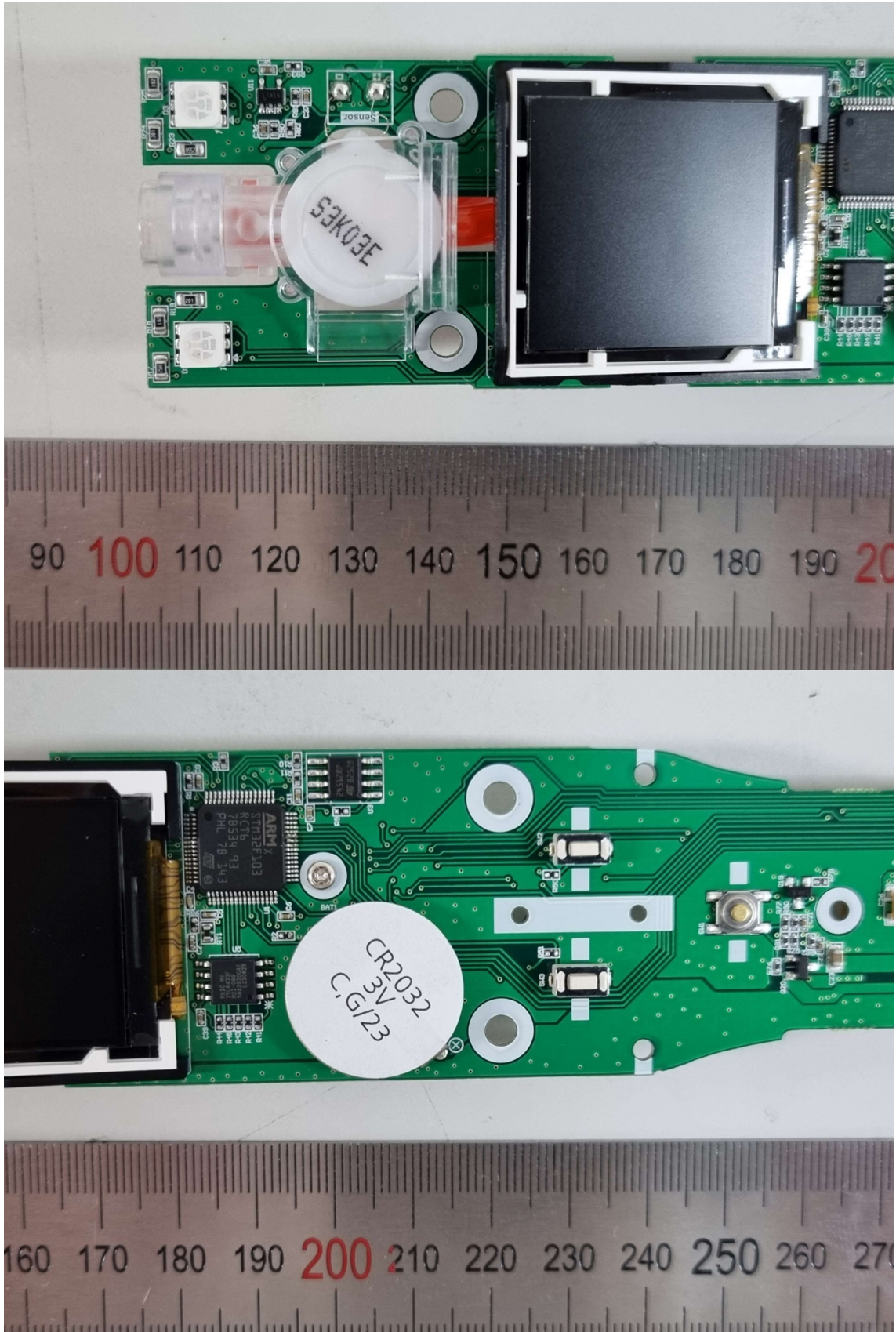
Main Board(Front, Scale up)
