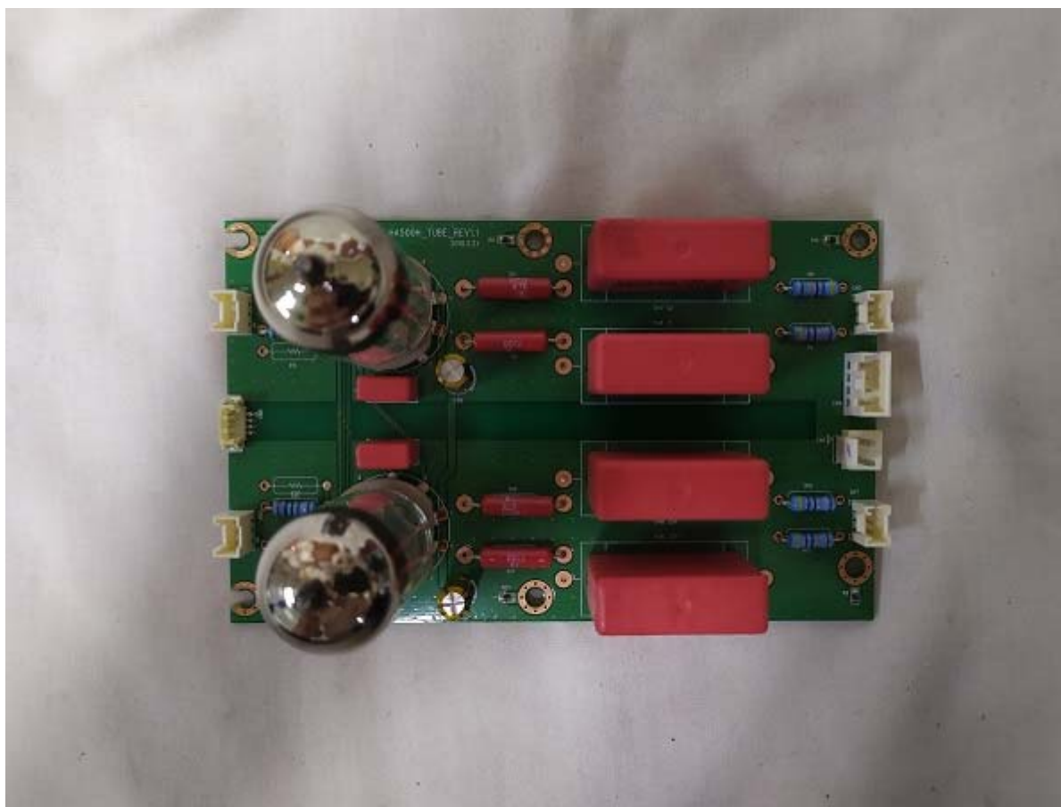
[Sub Board3 (Front)]
