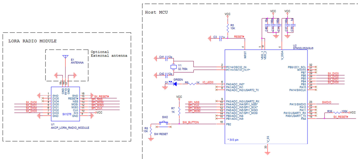
Peripheral Schematic
