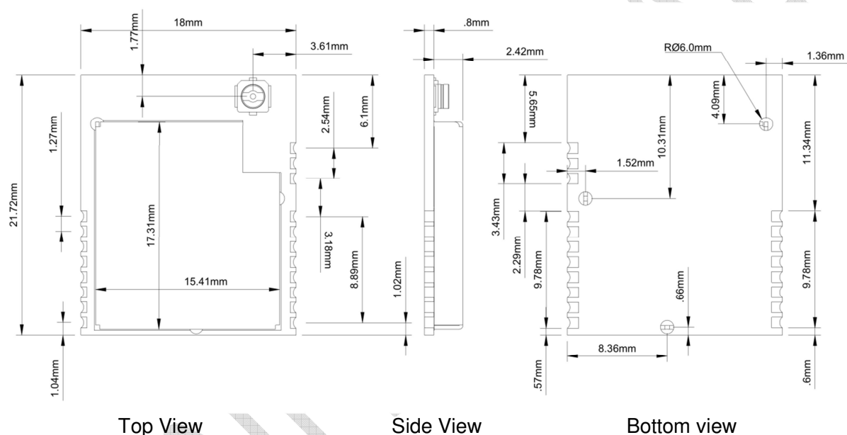
Mechanical dimensions
