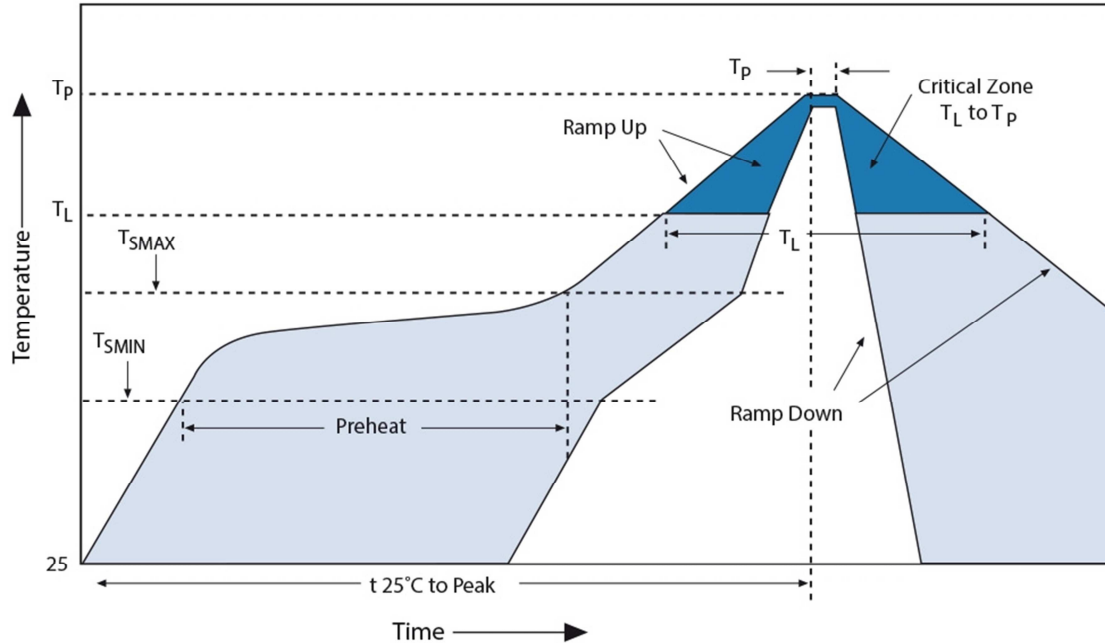
Lead-Free Reflow Profile Recommendation (IPC/JEDEC J-STD-020C)
