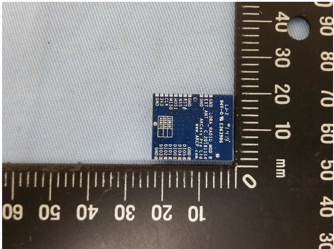
External Antenna
