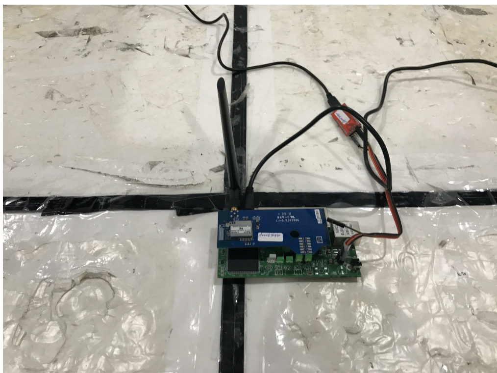
Photograph 4: Set-up for Spurious Emissions (Zoom In)
