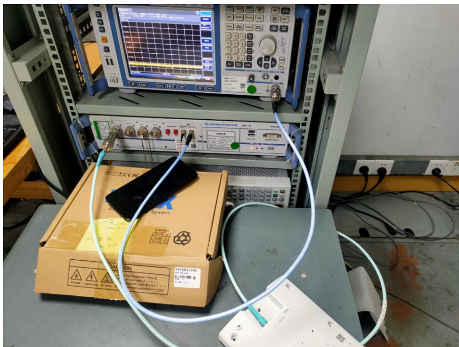
Photo of Radiated Emission Measurement (DFS)
