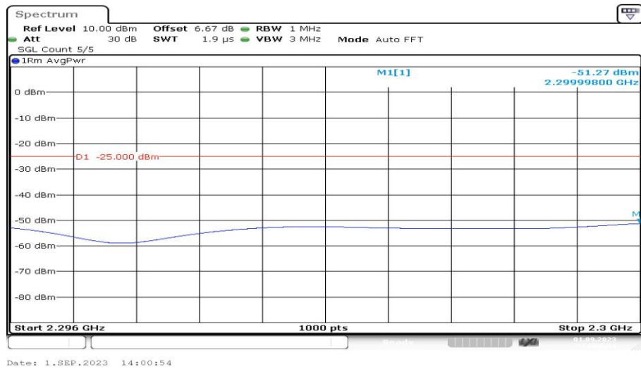
Band40-5MHz-QPSK-39175-1RB#0-Range7:2296~2300MHz-PASS
