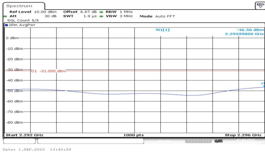
Band40-10MHz-16QAM-38750-1RB#0-Range6:2292~2296MHz-PASS
