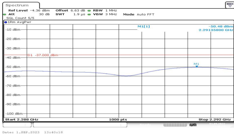
Band40-10MHz-16QAM-38750-1RB#0-Range5:2288~2292MHz-PASS
