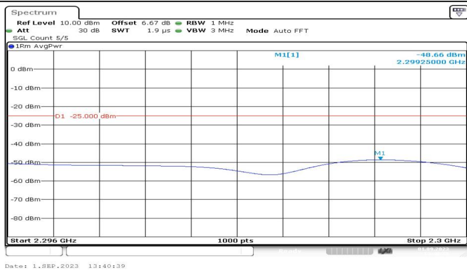
Band40-10MHz-16QAM-38750-1RB#0-Range7:2296~2300MHz-PASS
