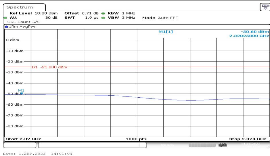
Band40-5MHz-QPSK-39175-1RB#0-Range8:2320~2324MHz-PASS
