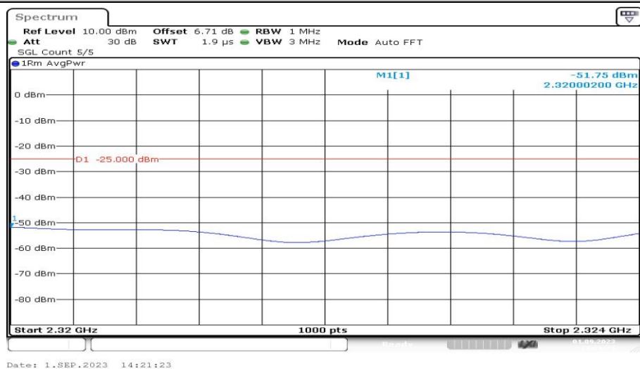
Band40-10MHz-QPSK-39200-1RB#0-Range8:2320~2324MHz-PASS
