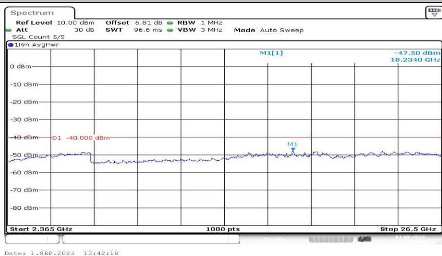
Band40-10MHz-16QAM-38750-1RB#0-Range16:2365~26500MHz-PASS
