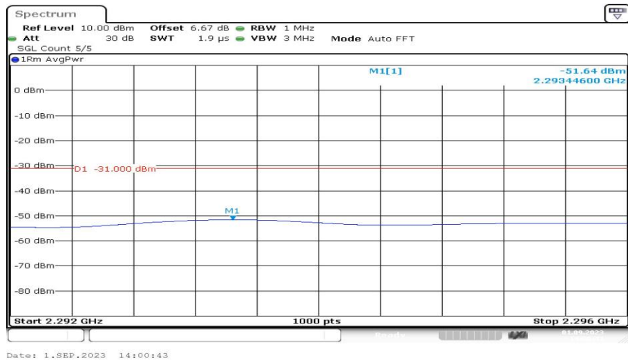
Band40-5MHz-QPSK-39175-1RB#0-Range6:2292~2296MHz-PASS
