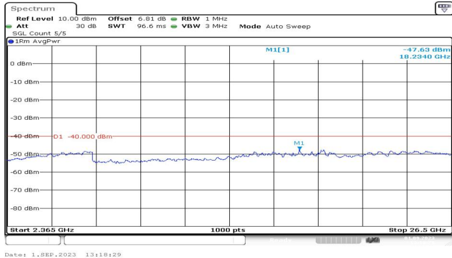
Band40-5MHz-16QAM-38775-1RB#0-Range16:2365~26500MHz-PASS
