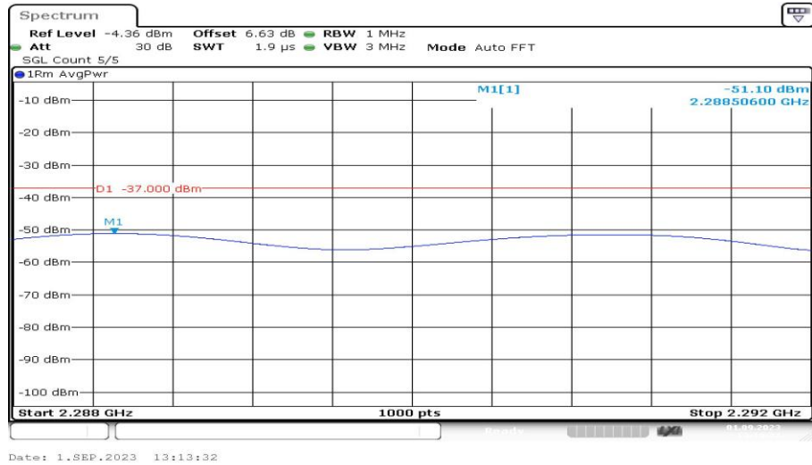
Band40-5MHz-QPSK-38775-1RB#0-Range5:2288~2292MHz-PASS
