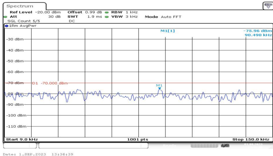
Band40-10MHz-QPSK-38750-1RB#0-Range1:0.009~0.15MHz-PASS
