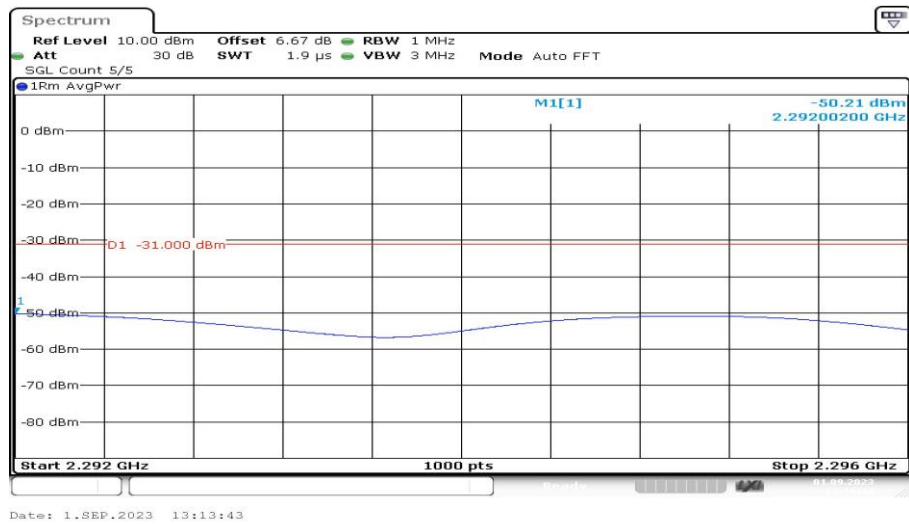
Band40-5MHz-QPSK-38775-1RB#0-Range6:2292~2296MHz-PASS
