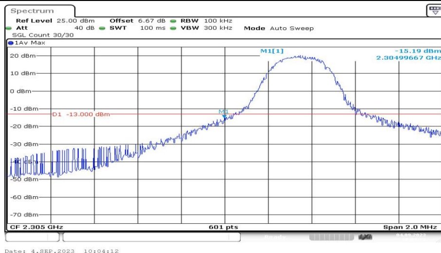
Band40-5MHz-QPSK-38725-1RB#0-PASS
