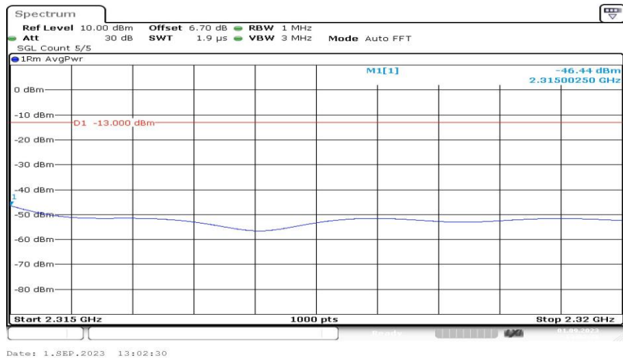
Band40-5MHz-QPSK-38725-1RB#0-Range9:2315~2320MHz-PASS
