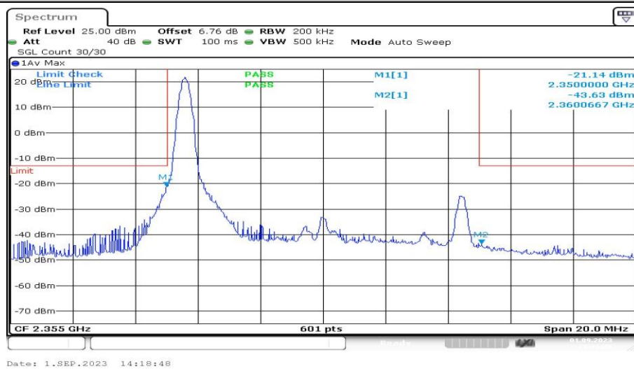
Band40-10MHz-16QAM-39200-1RB#0-PASS
