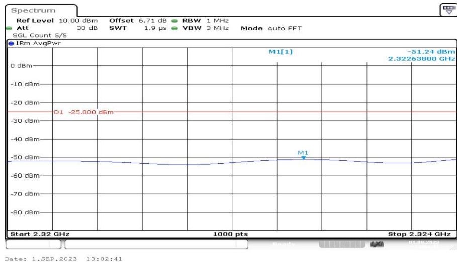
Band40-5MHz-QPSK-38725-1RB#0-Range10:2320~2324MHz-PASS
