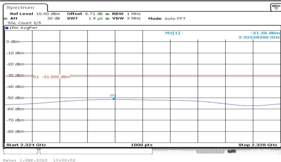
Band40-5MHz-QPSK-38725-1RB#0-Range11:2324~2328MHz-PASS
