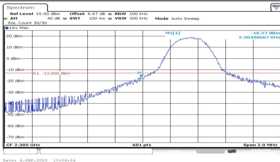
Band40-5MHz-16QAM-38725-1RB#0-PASS
