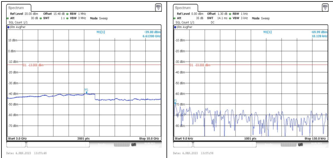
Band5_5MHz_QPSK_20425_1RB#0_3000~1000 Band5_5MHz_16QAM_20425_1RB#0_0.009~0.15 0_3000~10000 _0.009~0.15
