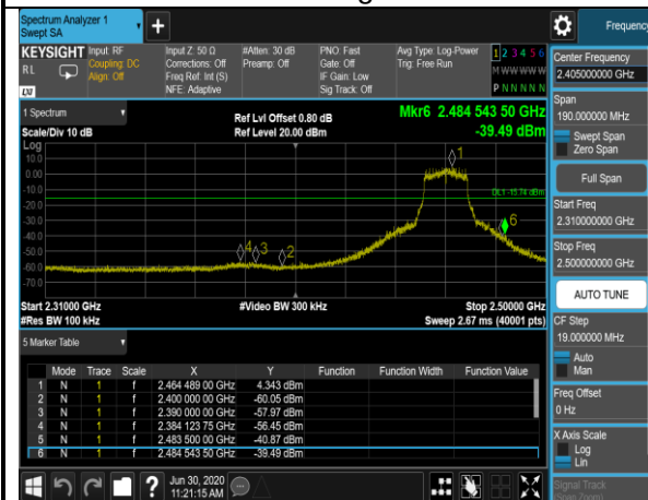
802.11g,2462MHz,Ant1,Plot 2,Band Edge
