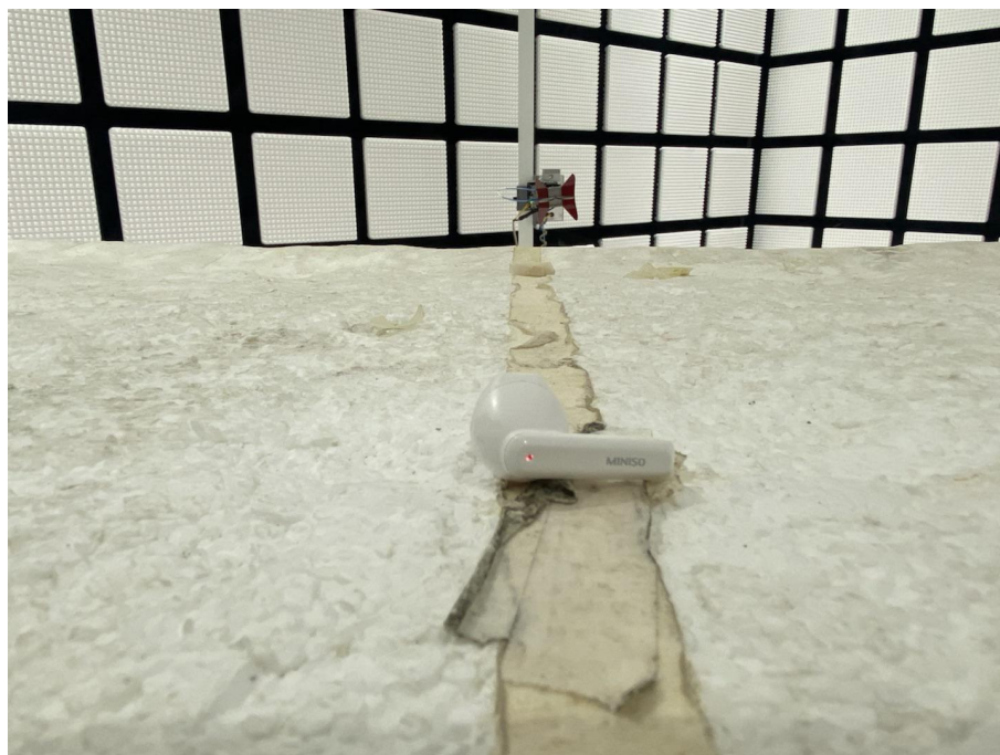
Radiated spurious emission Test Setup-4(Above 1GHz) Close-up
