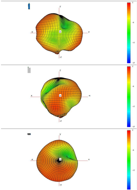
3D Radiation Pattern for 2450MHz
