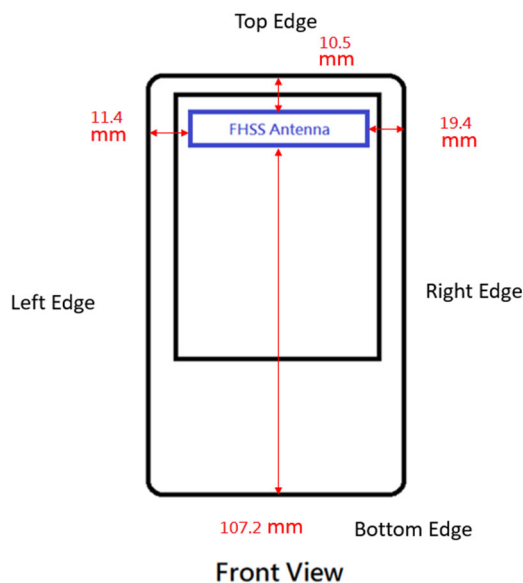
Photograph 13. Antenna position of EUT
