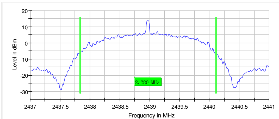
99 % Bandwidth
