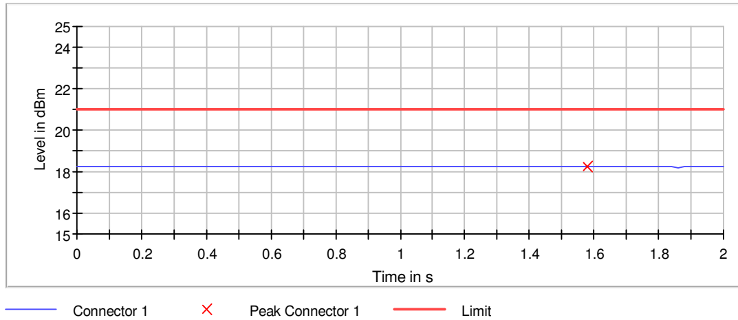
Peak Power
