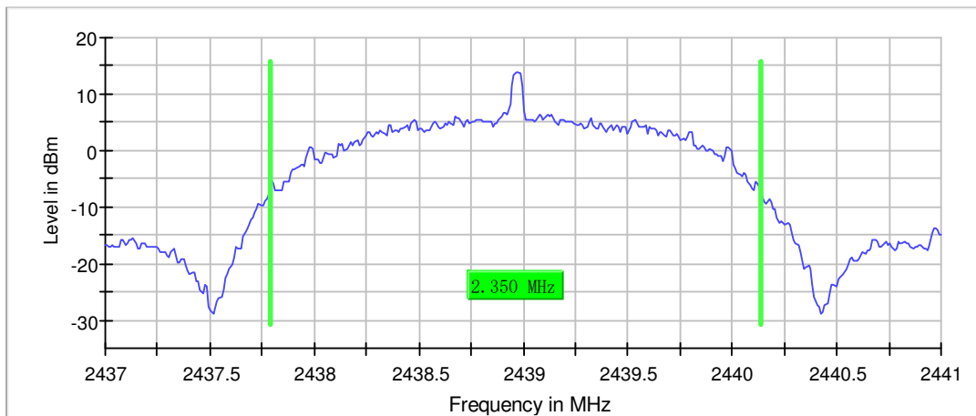
20 dB Bandwidth
