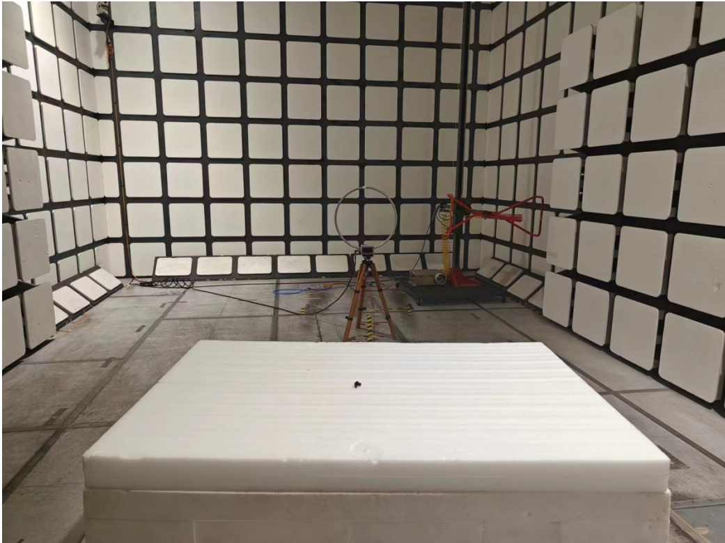
Radiated Emissions View (9kHz- 30MHz)
